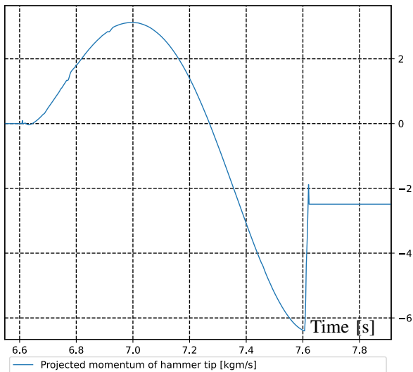
Fig. 5. Time evolution of the projected momentum along the normal \mathbf{n}
