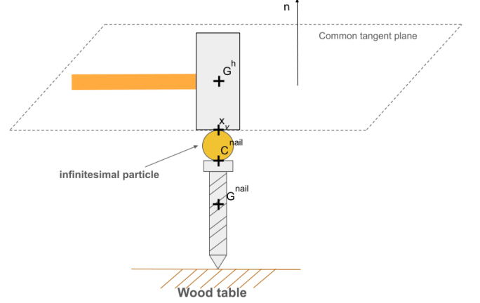
Fig. 1. Schematic of the collision using particle impact
