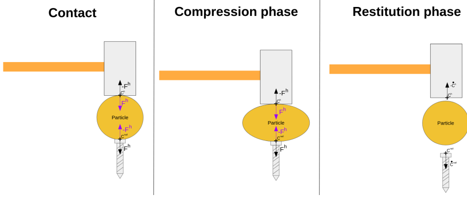
Fig. 2. Particle impact phases
