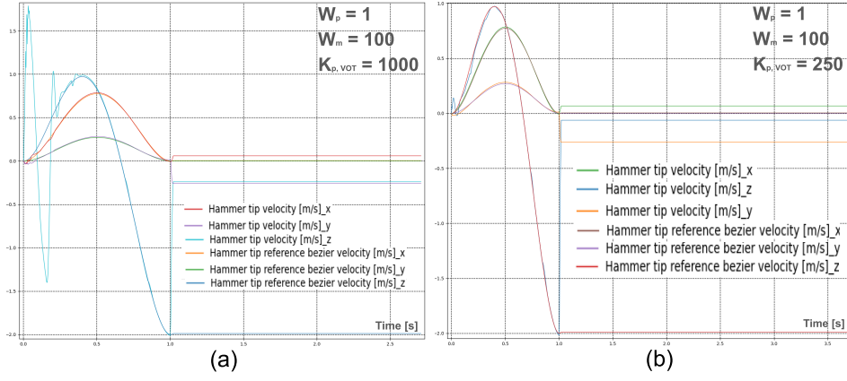
Fig. 3. Velocity tracking of the hammer tip for different K_{p,VOT} values
