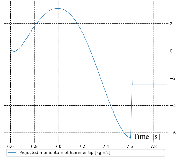
Fig. 5. Time evolution of the projected momentum along the normal \mathbf{n}
