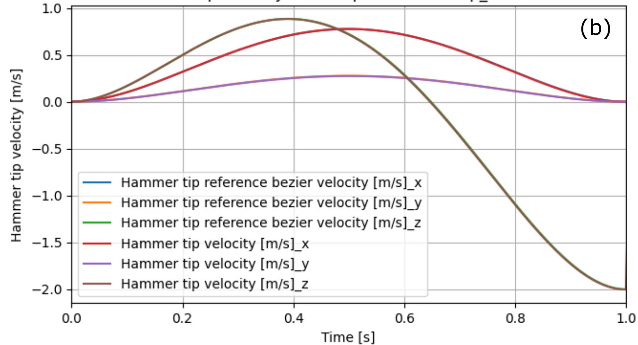
Hammer tip velocity with respect to time, K_p\_VOT = 100
