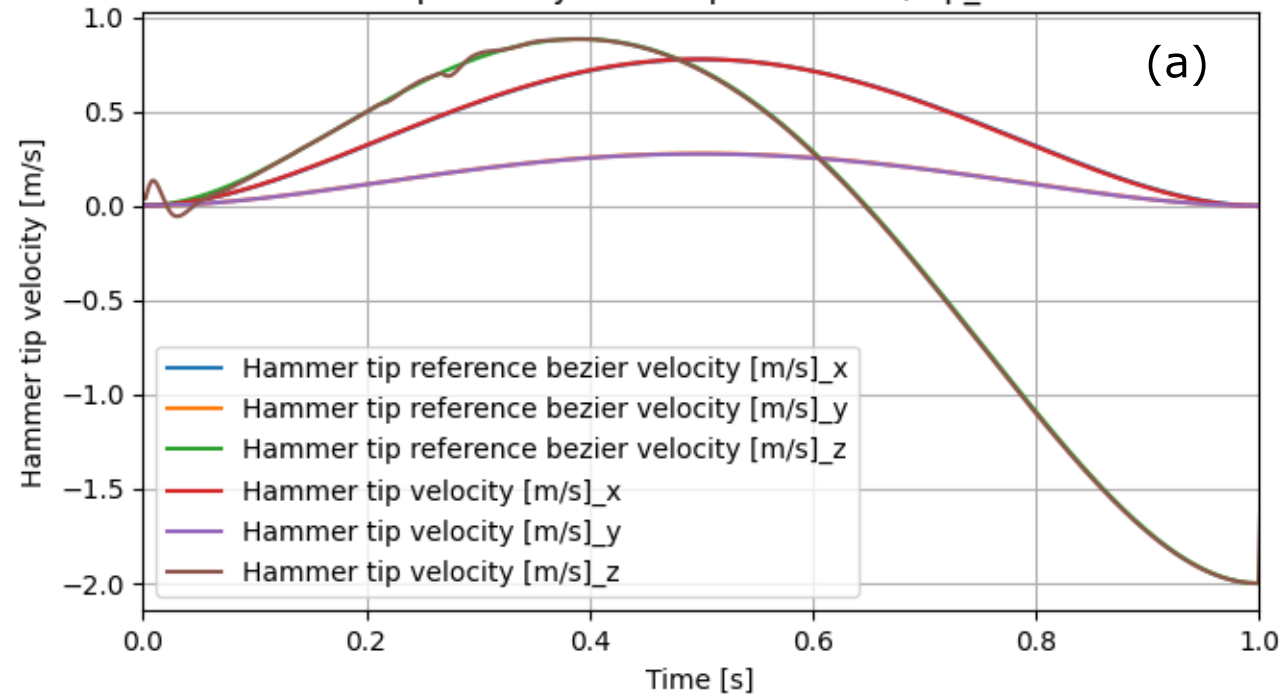
Hammer tip velocity with respect to time, K_p\_VOT = 250
