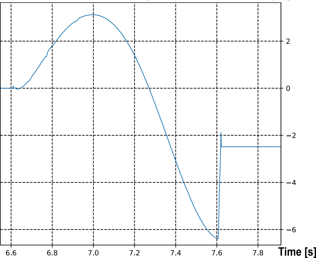
Projected momentum of hammer tip [kgm/s]
