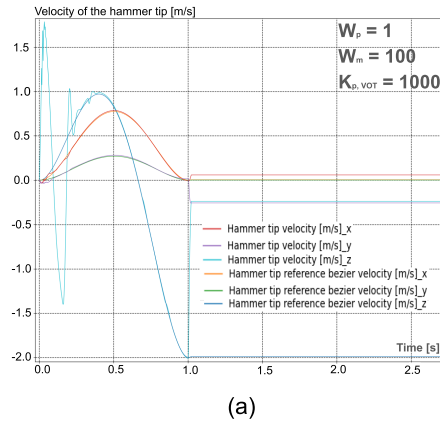
Fig. 4. Velocity tracking of the hammer tip for different K_{p,VOT} values.
