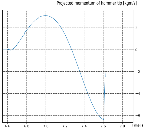
Fig. 3. Time evolution of the projected momentum along the normal \mathbf{n} .
