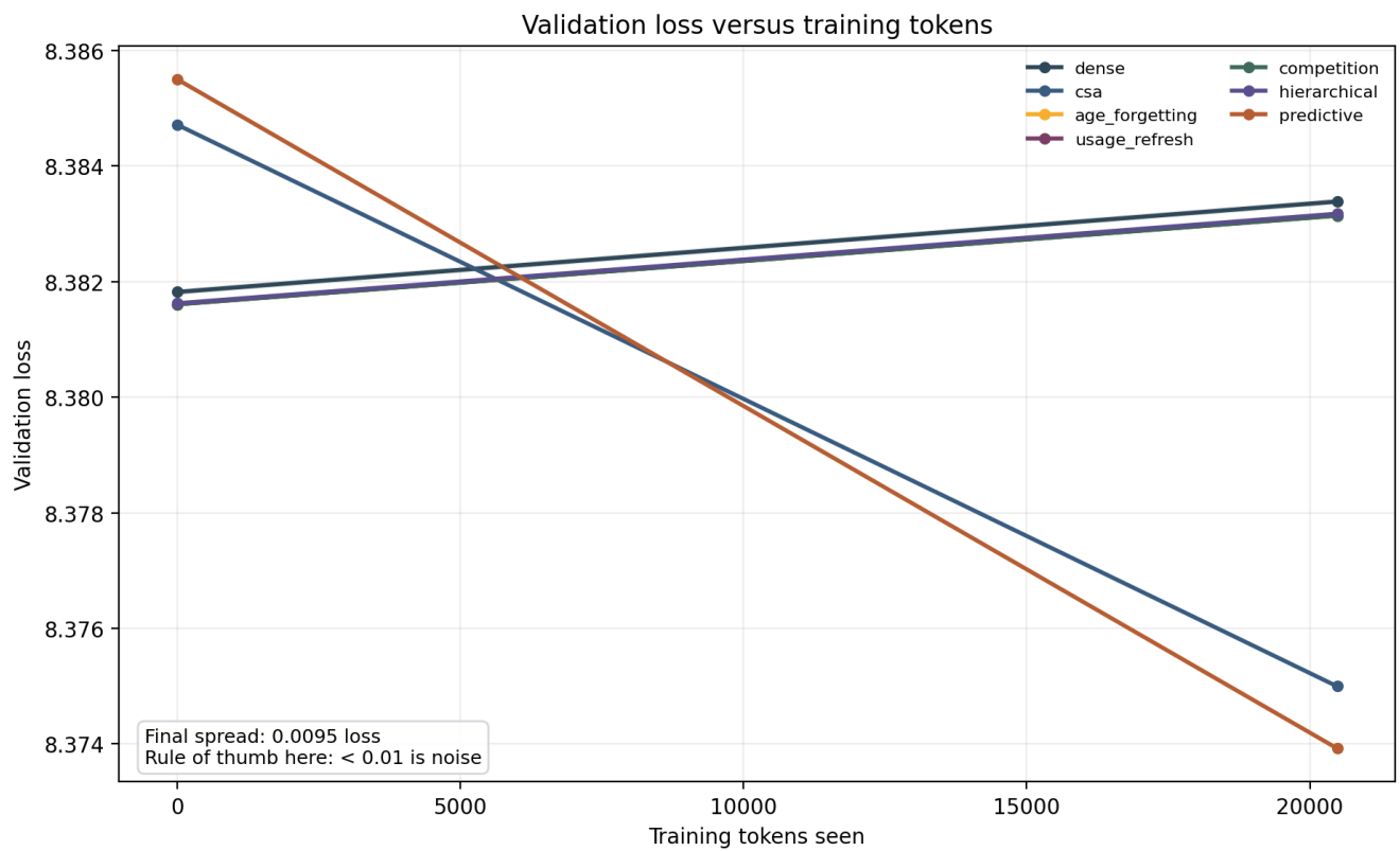
Figure 4: Validation loss versus training tokens on the 20k-token Mac pilot. The curves are nearly on top of each other, which makes the practical noise rule easy to see: differences smaller than about 0.01 loss at this scale are not yet convincing.
