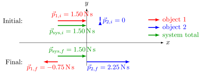
Figure 2: Vector diagram for Elastic 1 (momenta in N s)
