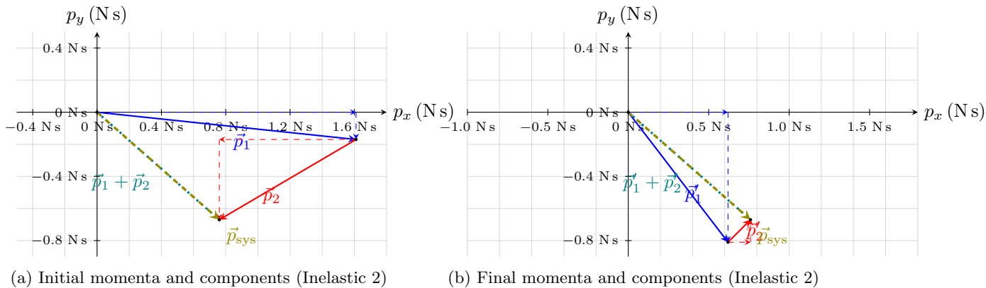
Figure 2: Tip-to-tail addition of components of momenta
