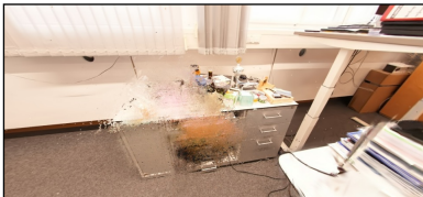
w/o QA-Mask
