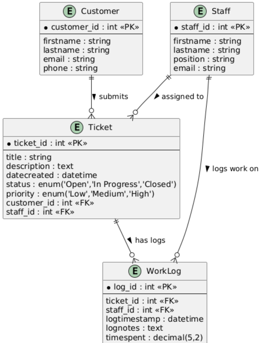
Figure 4: Assignment 2 – Relational Schema
