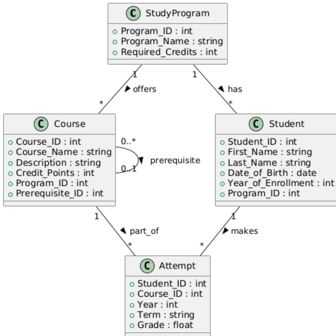
Figure 2: Assignment 1 – Relational Schema
