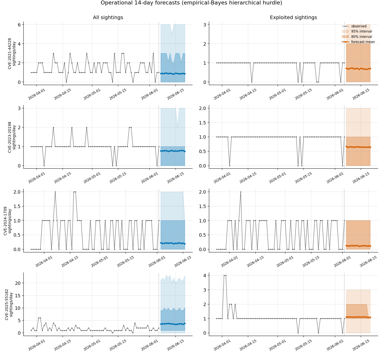
Figure 10: Out-of-sample 14-day forward forecasts for four actively-exploited CVEs, using the paper’s recommended models: the empirical-Bayes hierarchical hurdle on all sightings (left) and the type-specific pooled hurdle on the exploited stream (right). Grey: observed history; dotted line marks the last observation; coloured line is the forecast mean, with 80% and 95% predictive intervals shaded.
