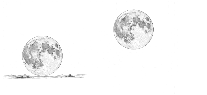
Figure 13 — The same moon, twice, drawn at the same diameter. Measured on the plate the two discs differ by under one per cent; everything else is the surrounding. The astronomer knows this and sees the left one as larger.
