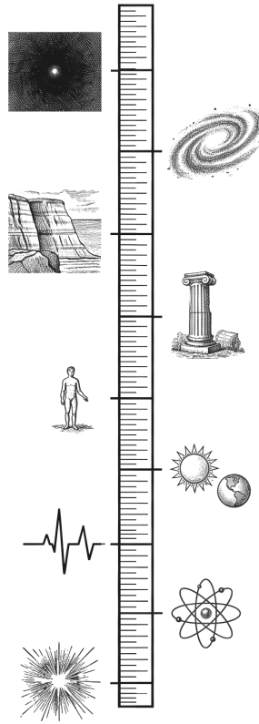
Figure 12 — The domain, as a scale. From a burst at the Planck tick, through an atom's vibration, a heartbeat, the day, a human life, recorded history, the stratigraphic record and a galaxy's turning, to a single point of light in emptiness. The column is logarithmic; the present epoch sits nowhere near the top.
