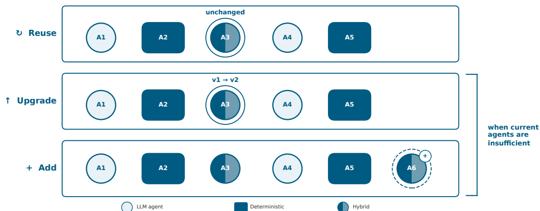
Figure 3.1: The agent library supports three operations: reuse an existing agent unchanged, upgrade it as a task-specific version, or add an agent for a missing capability.
