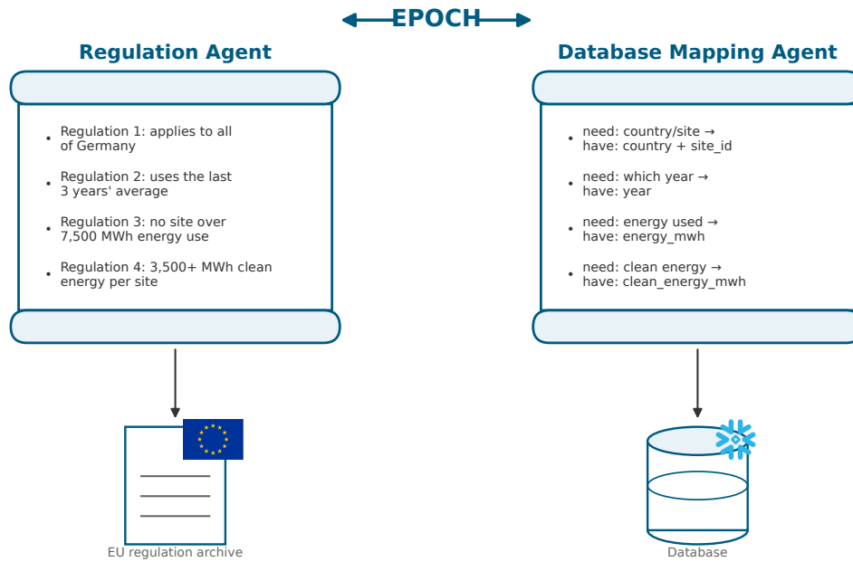
Figure 3.2: The isolated memory shelf system. A regulation-analysis role reads the European Union regulation archive, while a database-mapping role reads the operational catalog and receives only the approved regulatory handoff. Neither role can reach the other's source. The implementation codes visible in the figure are mapped to their full contracts in Appendix D. The rules and data answers are illustrative, not the recorded output of an actual pipeline run.
