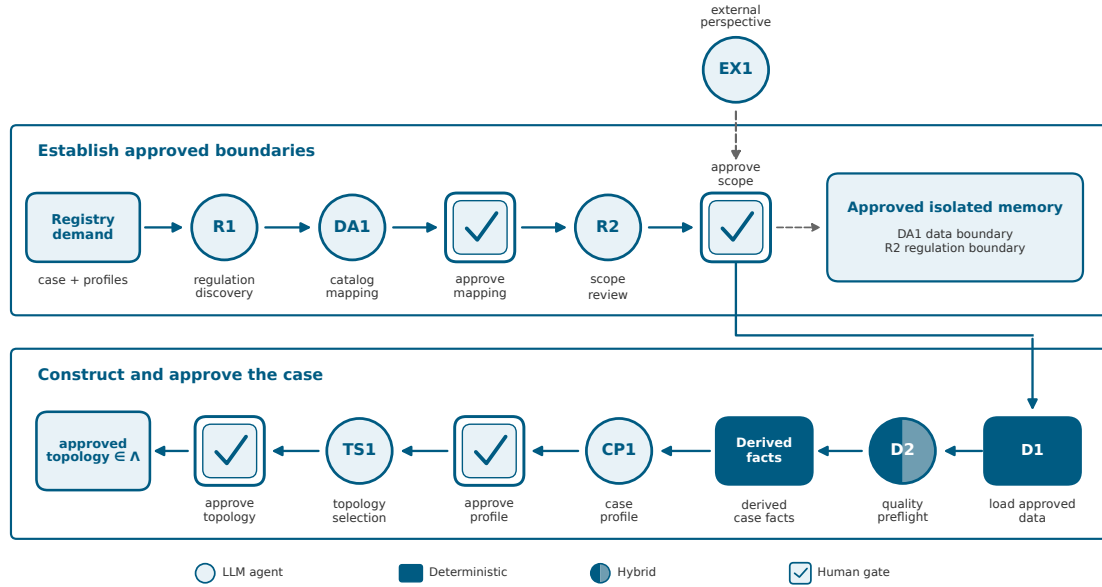
Figure 3.4: Agent and human-gate sequence that turns a registry demand into an approved topology in \Lambda , using UC2.1 as the working example. External commentary reaches the scope-approval gate as advisory evidence and does not enter the isolated memory. The anonymized execution behind Figure 3.4 can be inspected from its Stage 1 overview at https://emrecanulu.com/epoch/uc2-1/overview/ .
