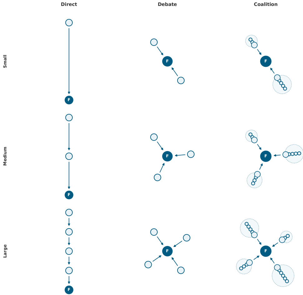
Figure 2.6: Each topology family admits several agent-count configurations without changing shape, and every configuration feeds the same centred finalizer role ( F ). Direct remains one ownership chain whether it runs two, three, or five dependent steps. Debate still reconciles independent readings of one claim whether two, three, or four readers take part. Coalition is the deliberate exception: domain islands are never the same size, so each example combines differently sized domains, all converging through their own local hub. The configurations shown are illustrative examples, not recorded pipeline runs.
