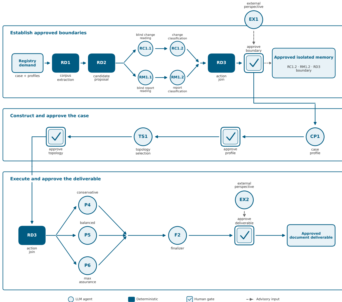
Figure 3.6: UC4's complete chain: Stage 1 boundary construction (top), case construction (middle), and Stage 2 topology-bound execution (bottom), from registry demand to the approved document deliverable.
