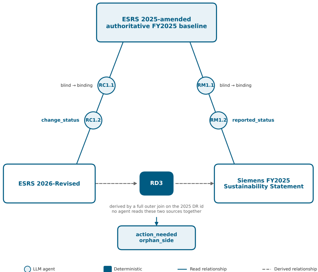
Figure 3.7: UC4’s registry compares three sources: the 2025-amended ESRS baseline, the 2026-Revised ESRS , and Siemens’ FY2025 Sustainability Statement . The 2025 baseline sits at the apex because it is the shared key both real comparisons join on: RC1.1 \rightarrow RC1.2 produces change_status against the 2026 text, and RM1.1 \rightarrow RM1.2 produces reported_status against the Siemens statement. The dashed base edge marks the relationship no agent reads directly. RD3 derives it by joining the two verdicts on the 2025 disclosure-requirement id, producing action_needed and orphan_side .
