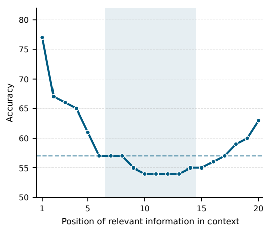
Figure 2.1: Accuracy is highest for information at the start or end of the context and drops in the middle. Adapted from Du and colleagues [2].
