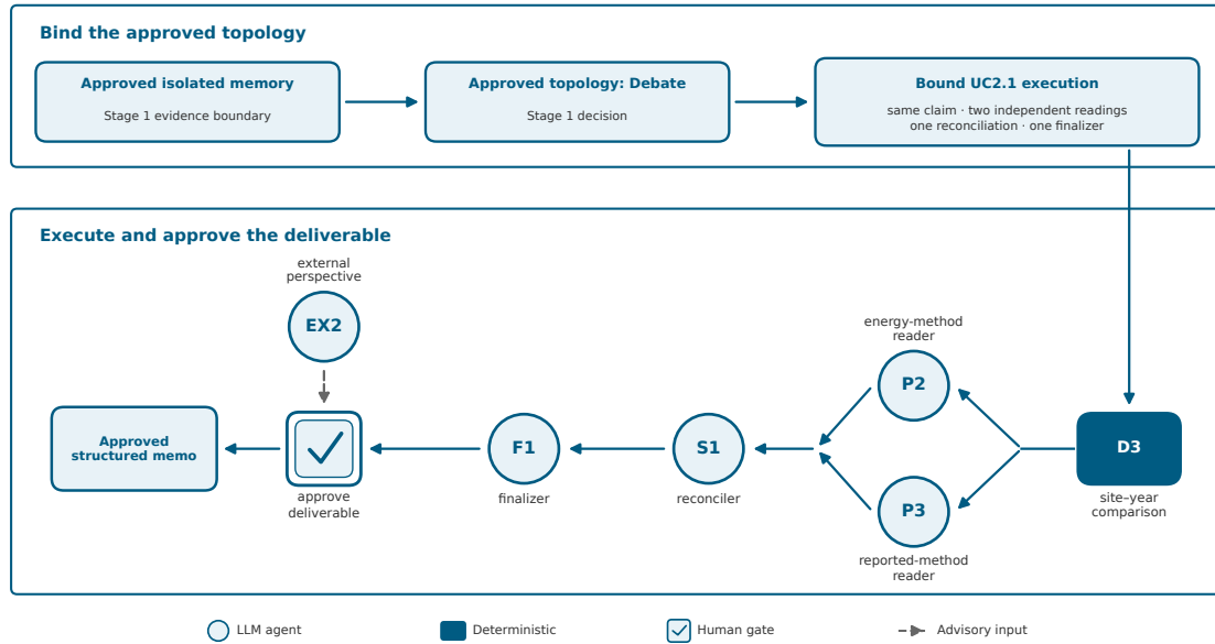
Figure 3.5: UC2.1 Stage 2 execution after the approved Debate selection. The deterministic comparison branches into two independent method readings, which first meet at reconciliation. The finalizer converts that record into the requested structured memo. External commentary reaches the human gate as advisory evidence and does not enter the approved deliverable. Its topology-bound continuation is available in the corresponding Stage 2 overview at https://emrecanulu.com/epoch/uc2-1/stage2/ .
