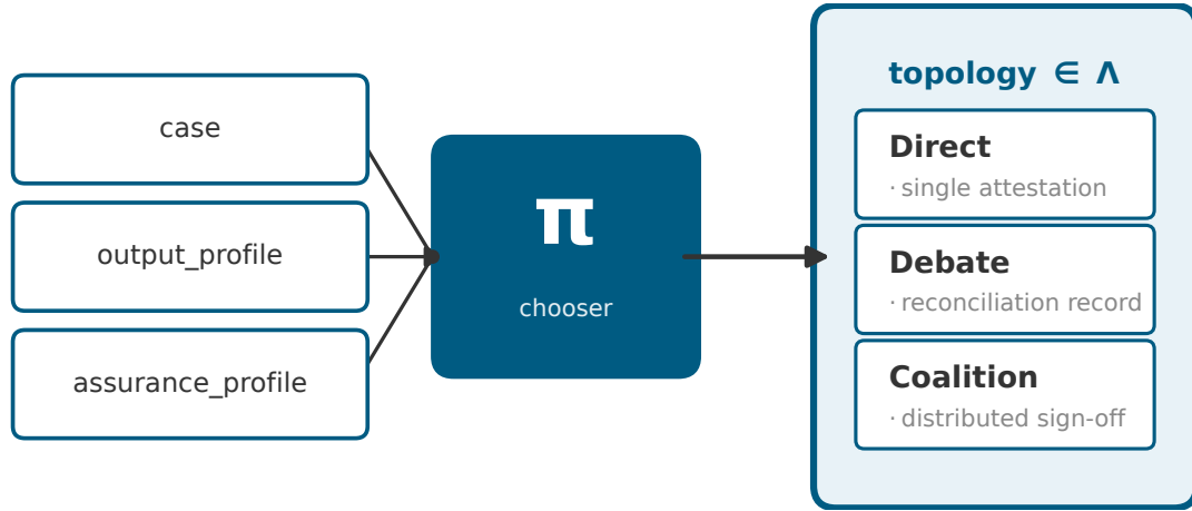
Figure 2.7: EPOCH's selector \pi maps the approved case profile, namely case , output_profile , and assurance_profile , to a topology in the library \Lambda . Each topology carries a structurally distinct assurance artifact.
