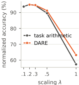
(b) 5 tasks: DARE vs TA
