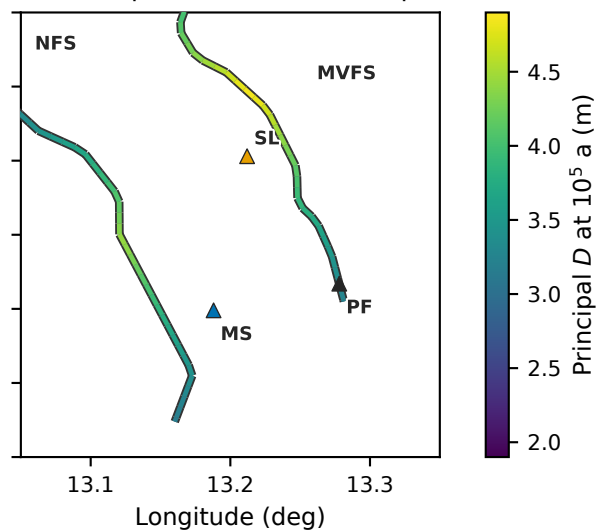
(b) 84th percentile hazard map
