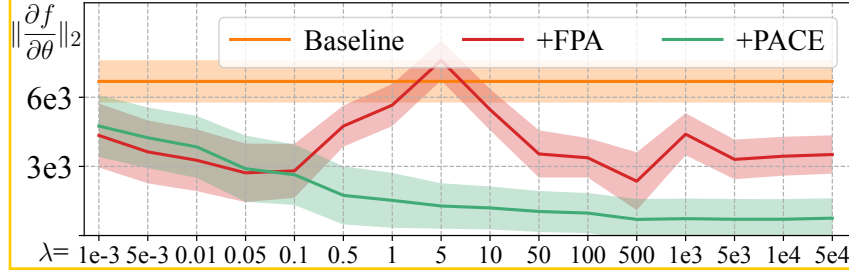
Figure 9: Gradient norms of models across wide range of regularization strengths \lambda on Camelyon (VTAB-1K) w/ Swin-B. Line and shadow represent mean and std over training epochs. While gradient explosion is less frequent for FPA in this setting, it exhibits unpredictable gradient norm with varied regularization strengths. In contrast, PACE reliably lowers gradient norms as regularization strength \lambda increases, demonstrating its robustness for effective gradient control.
