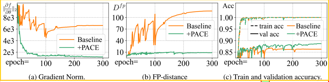
Figure 4: Analysis for PACE. (a) gradient norm, (b) FP-Distance and (c) train & val. accuracy are evaluated on the validation set of Camelyon (VTAB-1K) with baseline \text{LoRA}_{\text{mul}} + \text{VPT}_{\text{add}} on Swin-B.
