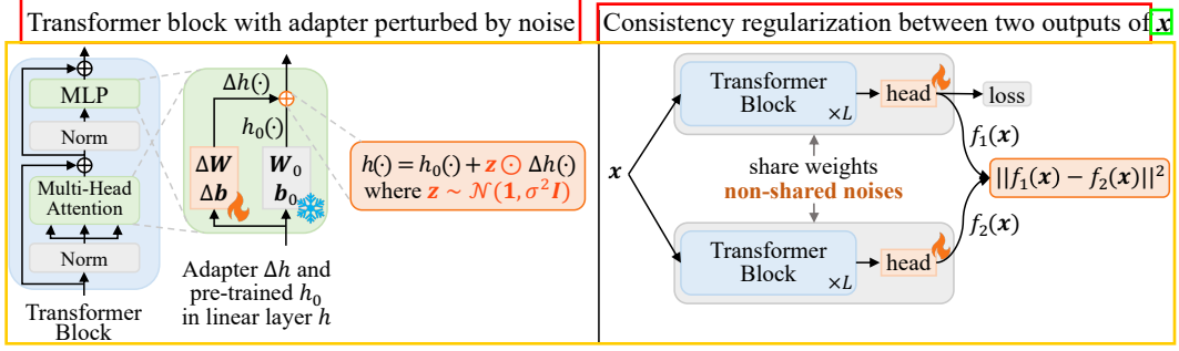
Figure 2: Our pipeline. Adapter \Delta h(\cdot) and h_0(\cdot) from pre-trained model form the linear layer h of Multi-Head Attention and MLP in fine-tuned model. We perturb \Delta h(\cdot) with multiplicative noise and ensure the network remains consistent to same inputs under varying perturbations.
