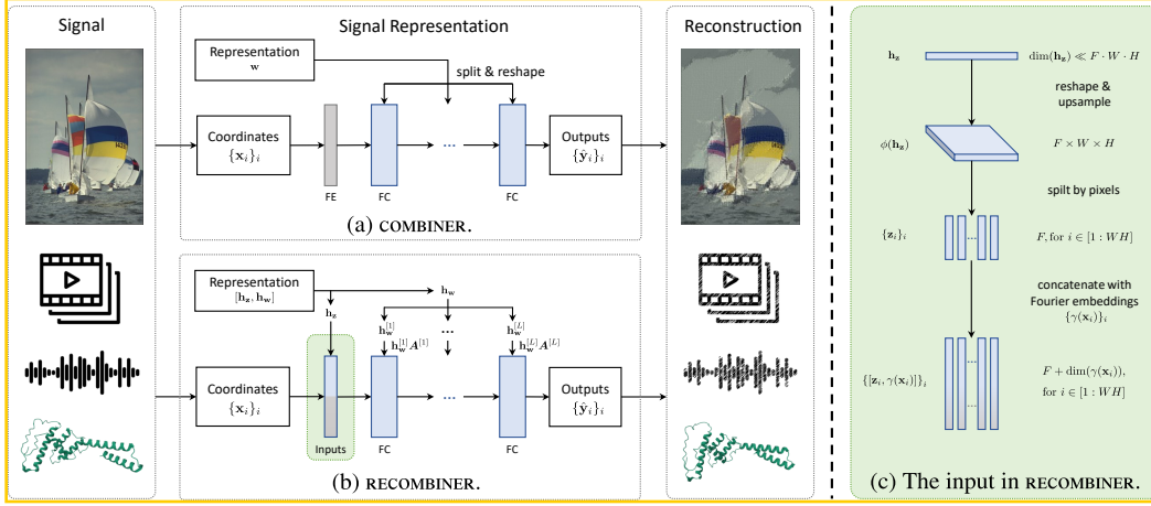
Figure 1: Schematic of (a) COMBINER and (b) RECOMBINER, our proposed method. See Sections 2 and 3 for notation. As the INR’s input, RECOMBINER uses h_w upsampled to pixel-wise positional encodings concatenated with Fourier embeddings. (c) A closer look at how RECOMBINER maps h_w to the INR input, taking images as an example. FE : Fourier embeddings; FC : fully connected layer.
