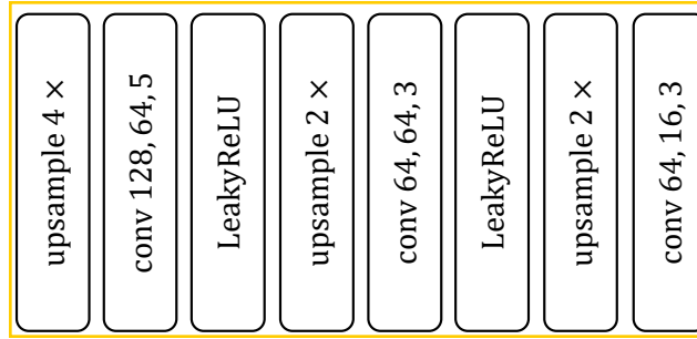
Figure 6: Architecture of the up-sampling network \phi for learnable positional encodings. The numbers in the convolution layer represent the number of input channels, the number of output channels, and kernel size respectively. same padding mode is used in all convolution layers. The kernel dimension depends on the modality, for instances, we use kernels with sizes of 5, 3, 3 for audio and proteins, kernels with sizes of 5 \times 5 , 3 \times 3 , 3 \times 3 for images, and kernels with sizes of 5 \times 5 \times 5 , 3 \times 3 \times 3 , 3 \times 3 \times 3 for video.
