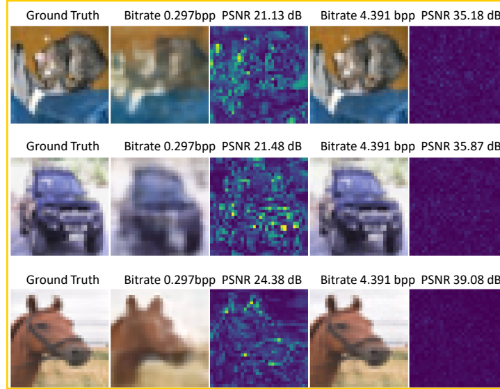
Figure 14: Decoded CIFAR-10 images and residuals.
