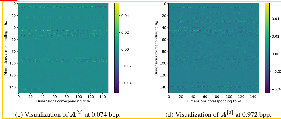
Figure 7: Visualizations.
