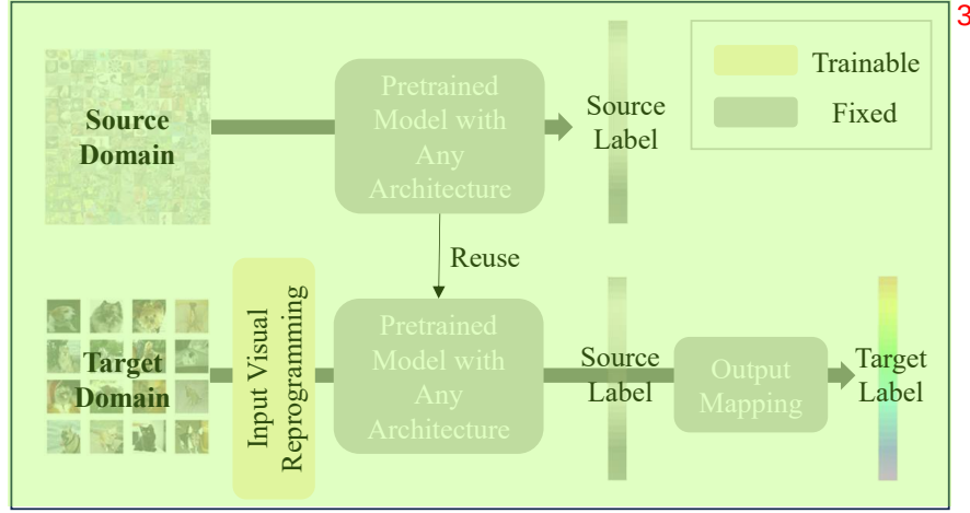
Figure 7. Problem setting of input visual reprogramming. The upper part shows the source task, while the lower part shows the target task. The main focus of visual reprogramming is the trainable part marked with a yellow rectangle in the input space.
