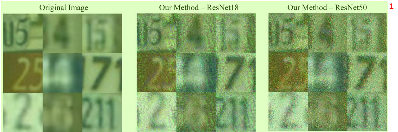
Figure 15. Original Images and Visual Reprogramming Results on SVHN 2
