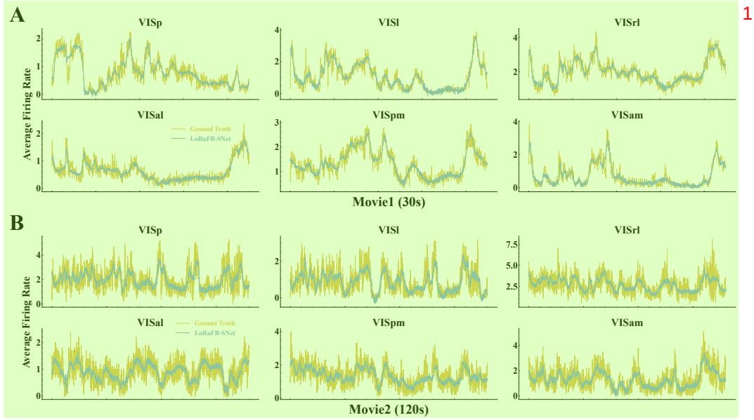
Figure 6: The real and regressed temporal profiles of individual biological neurons. We choose one neuron in each cortical region as an example.
