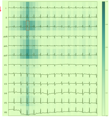
Figure 5: An illustration of an attention map. Attention scores from each encoder layer and head are averaged. 6
