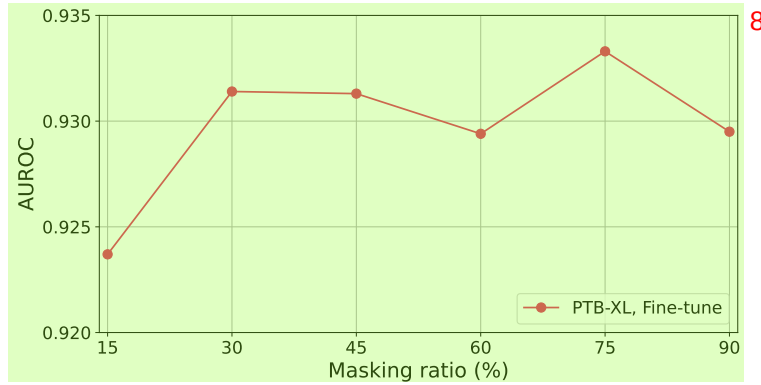
Figure 7: Ablation on masking ratio.
