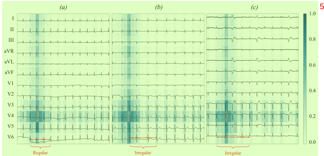
Figure 8: Self-attention maps of ECGs with regular and irregular rhythm. (a) is from a regular rhythm ECG, while (b) and (c) are from irregular rhythm ECGs. Pre-trained ST-MEM consistently assigns high attention weights to temporal patches that share a similar shape to the query patch. 6
