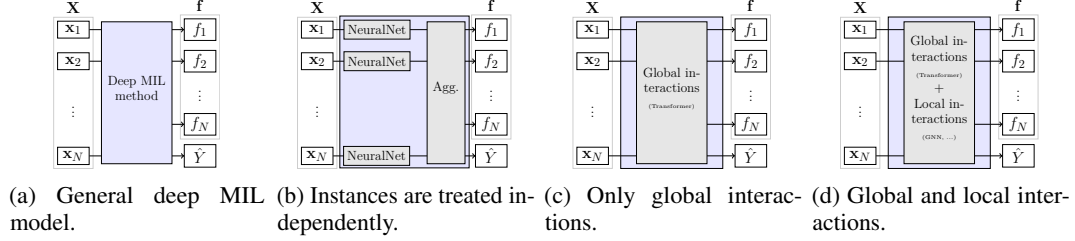
Figure 1: (a) Unified view of deep MIL models. Depending on how instances interact with each other in (a), we devise three different families of methods: (b), (c), (d).
