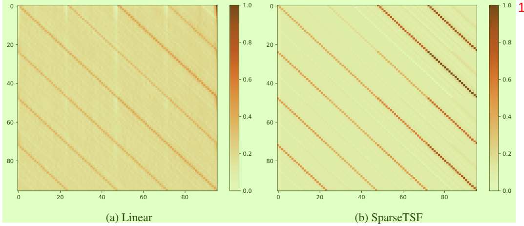
Figure 4: Visualization of normalized weights of the model trained on the ETTh1 dataset with both look-back length (X-axis) and forecast horizon (Y-axis) of 96.
