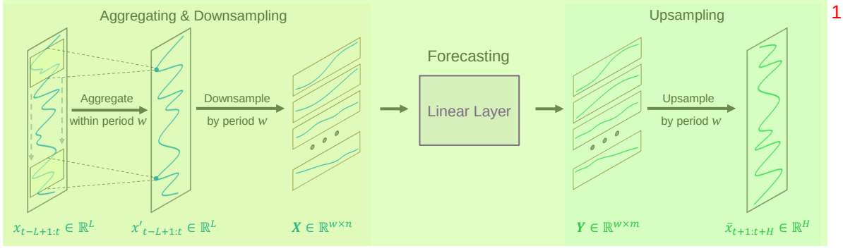
Figure 2: SparseTSF architecture.
