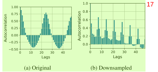
Figure 6: Comparison of autocorrelation in original and downsampled subsequences for the last channel in the Traffic dataset.
