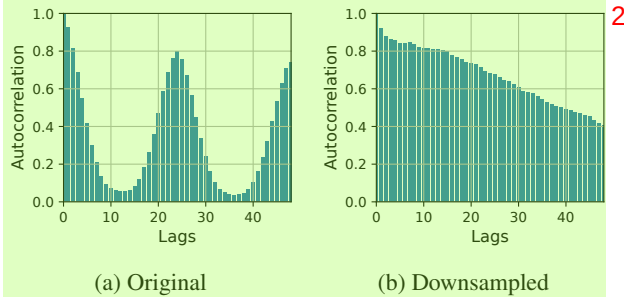
Figure 3: Comparison of autocorrelation in original and downsampled subsequences for the first channel in the ETTh1 dataset.
