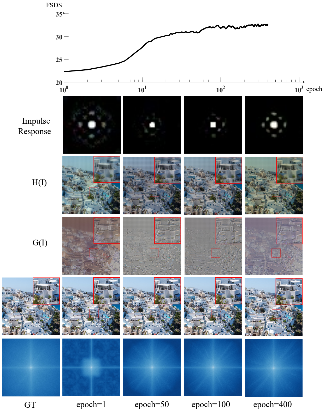
Figure 19. N(I) , H(I) and G(I) from different epoches during training.
