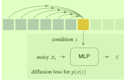
Figure 1: Diffusion Loss. Given a continuous-valued token x to be predicted, the autoregressive model produces a vector z , which serves as the condition of a denoising diffusion network (a small MLP). This offers a way to model the probability distribution p(x|z) of this token . This network is trained jointly with the autoregressive model by backpropagation. At inference time, with a predicted z , running the reverse diffusion procedure can sample a token following the distribution: x \sim p(x|z) . This method eliminates the need for discrete-valued tokenizers.
