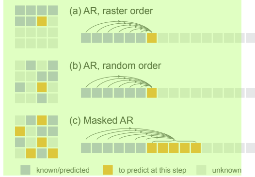
Figure 3: Generalized Autoregressive Models. 3
