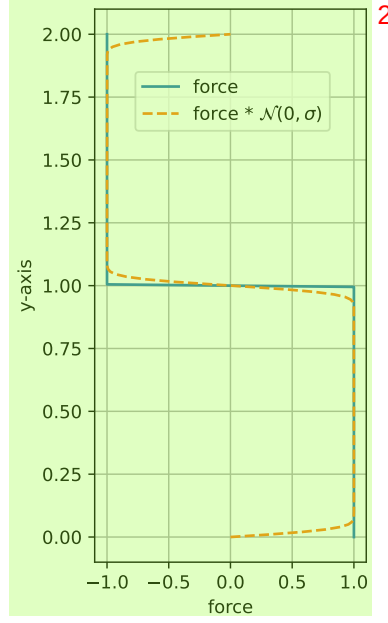
Figure 11. Forcing step function of the 2D reverse Poiseuille flow before (blue) and after convolution with normal distribution \mathcal{N}(0, 0.025^2) (orange).
