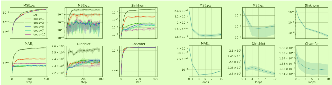
Figure 15. Ablations on LDC 2D with GNS-10-128 ( \alpha = 0.03 ) regarding the number of relaxation steps/loops. 8
