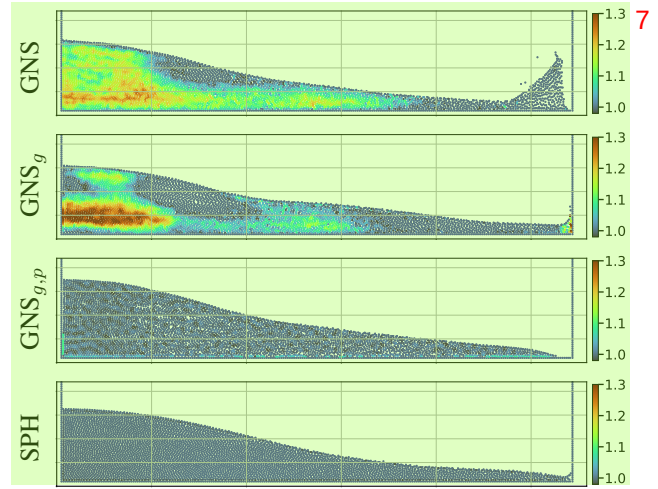
Figure 1. Neural SPH improves Lagrangian fluid dynamics, showcased by physics modeling of the 2D dam break example after 80 rollout steps. Different models exhibit different physics behaviors. From top to bottom: GNS (Sanchez-Gonzalez et al., 2020), GNS with corrected force only ( GNS_g ), full SPH enhanced GNS ( GNS_{g,p} ), and the ground truth SPH simulation. The colors correspond to the density deviation from the reference density; the system is considered physical within 0.98-1.02.
