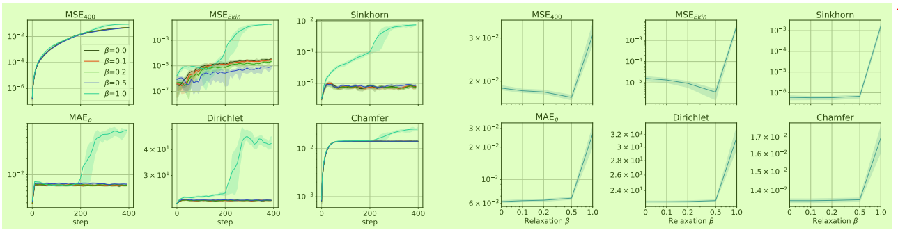
Figure 19. Ablations on LDC 2D with SEGNN-10-64 ( \alpha = 0.03 , l = 5 ) regarding relaxation parameter \beta . 8
