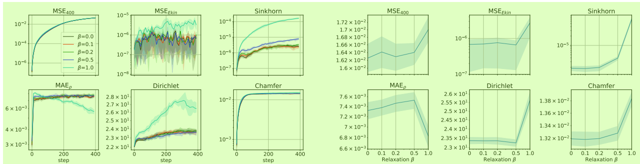
Figure 16. Ablations on LDC 2D with GNS-10-128 ( \alpha = 0.03 , l = 5 ) regarding relaxation parameter \beta . 10
