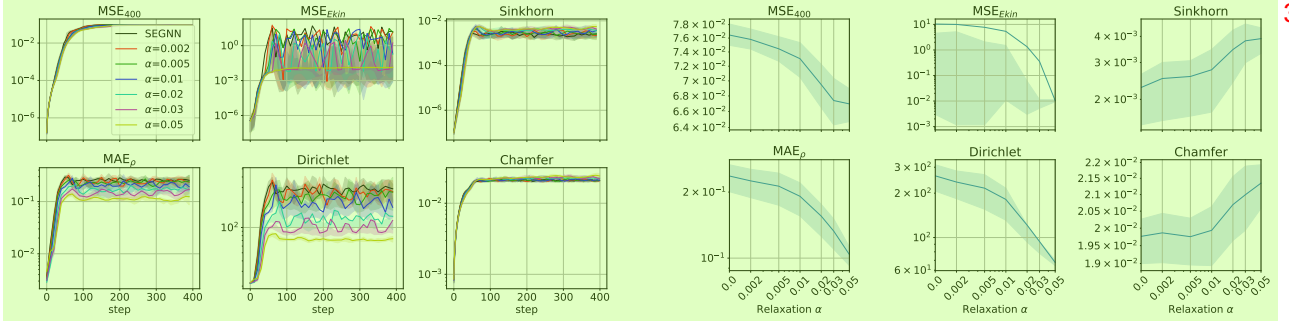
Figure 17. Ablations on LDC 2D with SEGNN-10-64 ( l = 1 ) regarding relaxation parameter \alpha . 4
