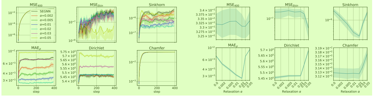
Figure 23. Ablations on LDC 3D with SEGNN-10-64 ( l = 1 ) regarding relaxation parameter \alpha . 3
