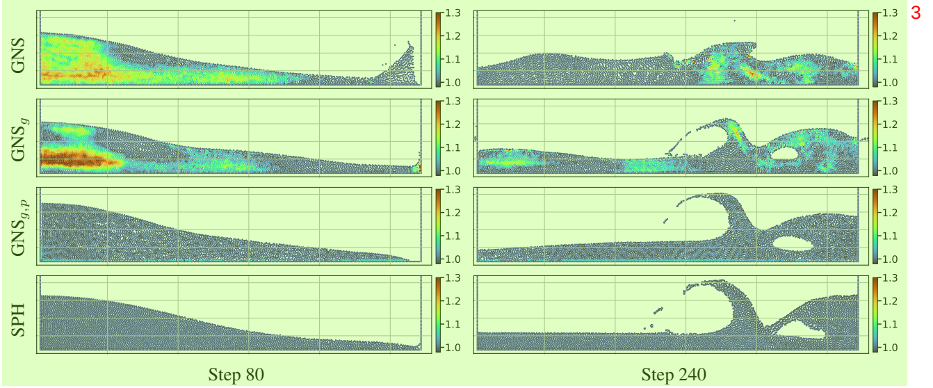
Figure 6. Dam break steps 80 and 240 of test rollout 0. Extends Fig. 1. 4
