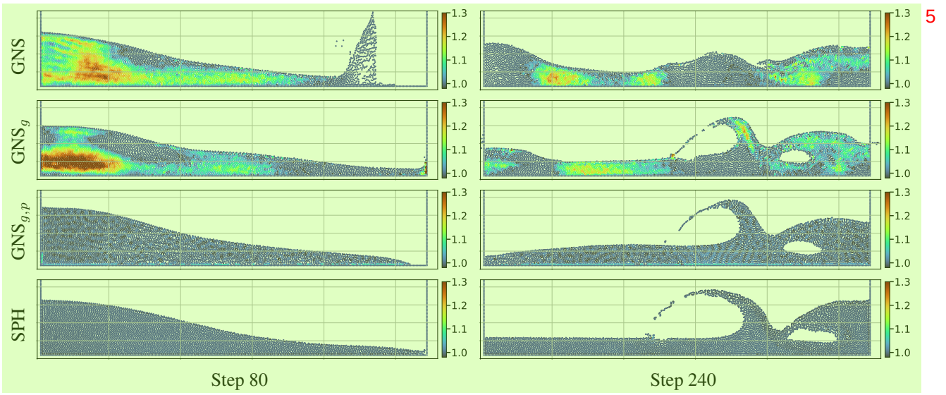
Figure 7. Dam break steps 80 and 240 of test rollout 13. 6
