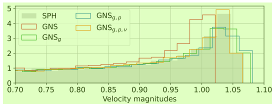
Figure 4. Velocity magnitudes histogram of 2D reverse Poiseuille 6 flow after 400 rollout steps (averaged over all rollouts). Our GNS_{g,p,\nu} matches the ground truth distribution of SPH.
