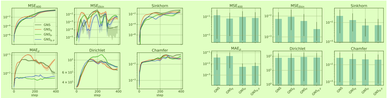
Figure 12. Ablations on DAM 2D with GNS-10-128 over the simulation length (left) and the average thereof (right). 10
