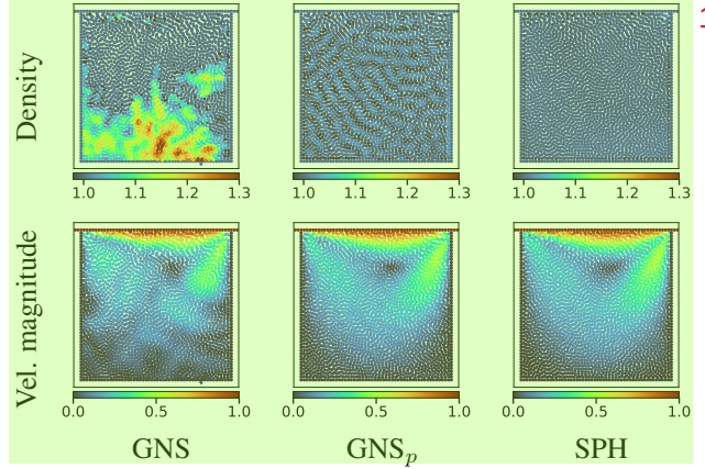
Figure 5. Density and velocity magnitude of 2D lid-driven cavity 11 after 400 rollout steps (left to right): GNS, GNS_p , SPH. The colors in the first row correspond to the density deviation from the reference density; the system is considered physical within 0.98-1.02.
