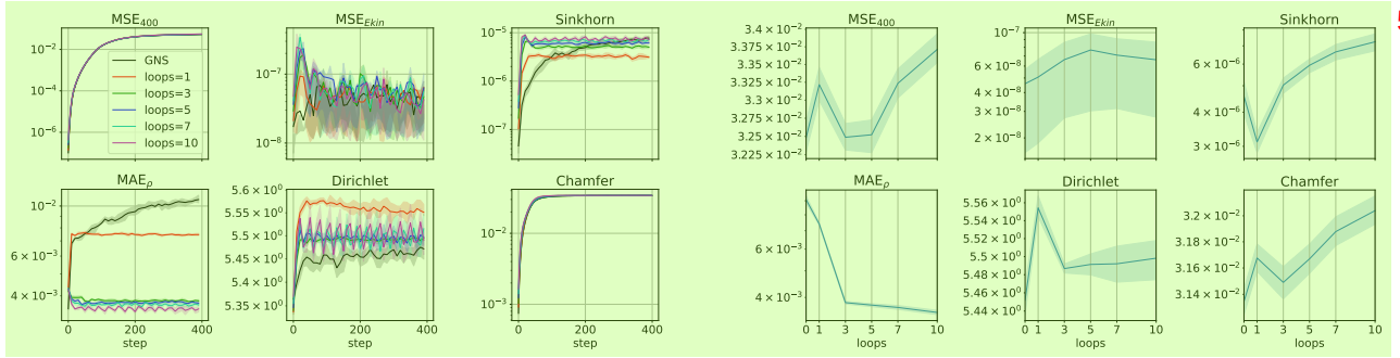
Figure 21. Ablations on LDC 3D with GNS-10-128 ( \alpha = 0.02 ) regarding the number of relaxation steps/loops. 6
