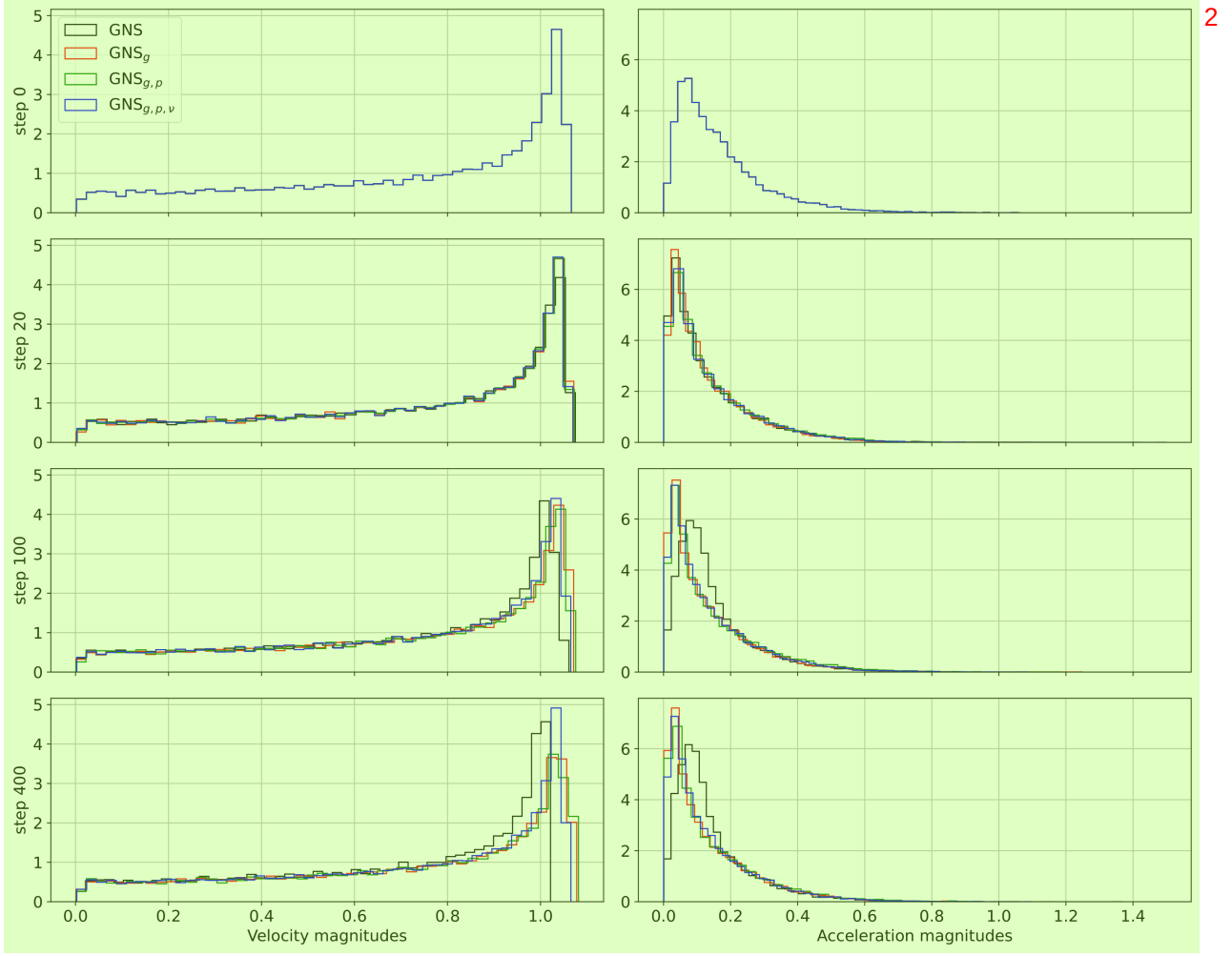
Figure 10. Velocity and acceleration magnitude histogram of 2D reverse Poiseuille flow after 400 rollout steps (average over all rollouts) 3 Extends Fig. 4.
