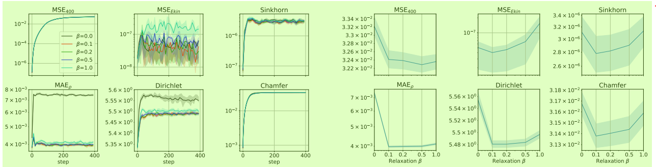
Figure 22. Ablations on LDC 3D with GNS-10-128 ( \alpha = 0.02 , l = 1 ) regarding relaxation parameter \beta . 8
