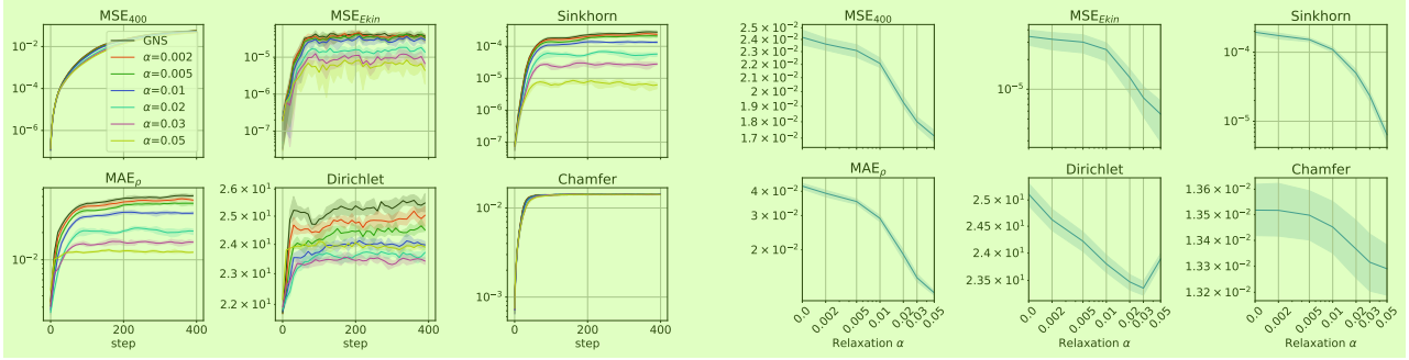
Figure 14. Ablations on LDC 2D with GNS-10-128 ( l = 1 ) regarding relaxation parameter \alpha . 6
