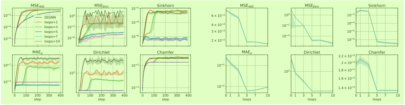
Figure 18. Ablations on LDC 2D with SEGNN-10-64 ( \alpha = 0.03 ) regarding the number of relaxation steps/loops. 6
