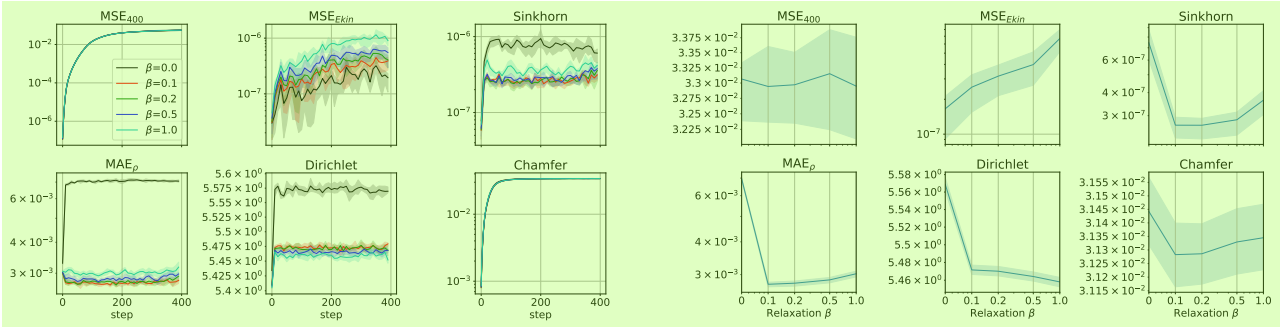
Figure 25. Ablations on LDC 3D with SEGNN-10-64 ( \alpha = 0.02 , l = 1 ) regarding relaxation parameter \beta . 7
