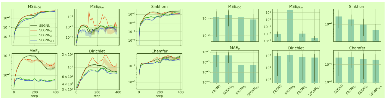
Figure 13. Ablations on DAM 2D with SEGNN-10-64 over the simulation length (left) and the average thereof (right). 12
