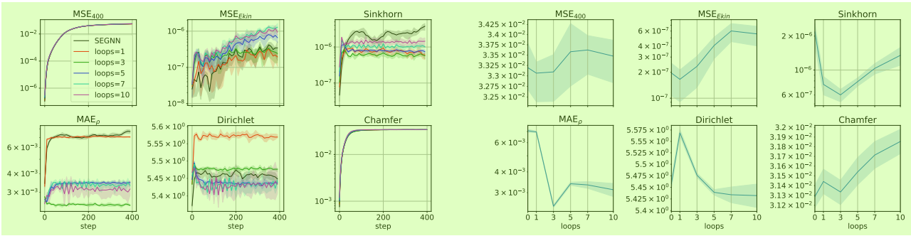
Figure 24. Ablations on LDC 3D with SEGNN-10-64 ( \alpha = 0.02 ) regarding the number of relaxation steps/loops. 5
