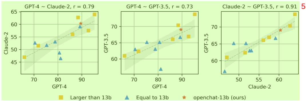
Figure 9: The consistency of three evaluators, GPT-4, GPT-3.5, Claude-2 in AlpacaEval benchmark. 6
