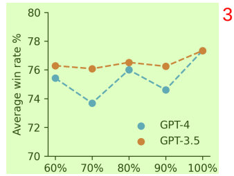
Figure 6: Effects of subsampling a specific class of data.
