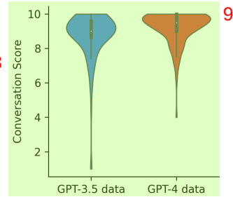
Figure 3: Quality distribution of GPT-3.5 and GPT-4 conversations in the ShareGPT dataset.
