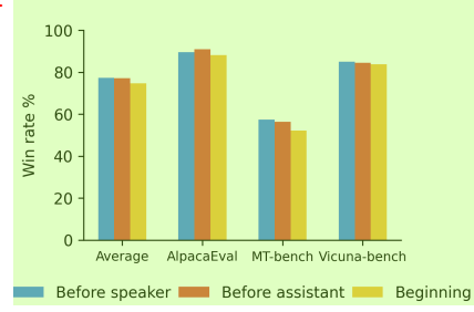
Figure 7: Effects of class-conditioned prompt tokens during training phase. 4
