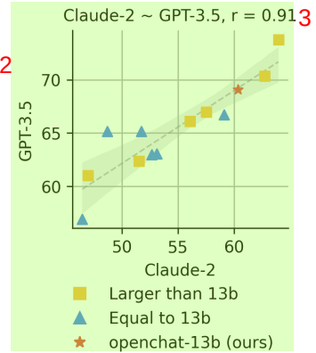
Figure 8: The consistency between GPT-3.5 and Claude-2 in AlpacaEval benchmark.
