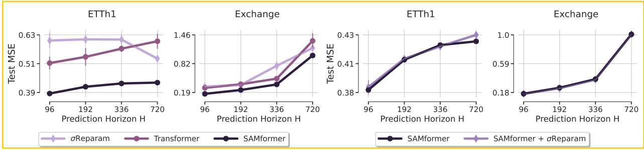
(a) Comparison of Transformer, \sigma Reparam and SAMformer. (b) Comparison of SAMformer and SAMformer + \sigma Reparam.
