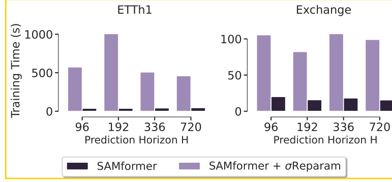
Figure 11: Using \sigma Reparam on top of SAMformer heavily increases the training time.
