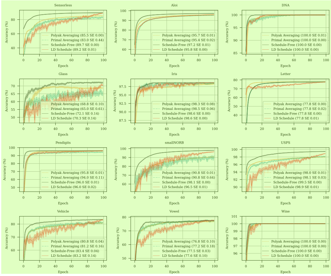
Figure 7: Stochastic logistic regression experiments. 2
