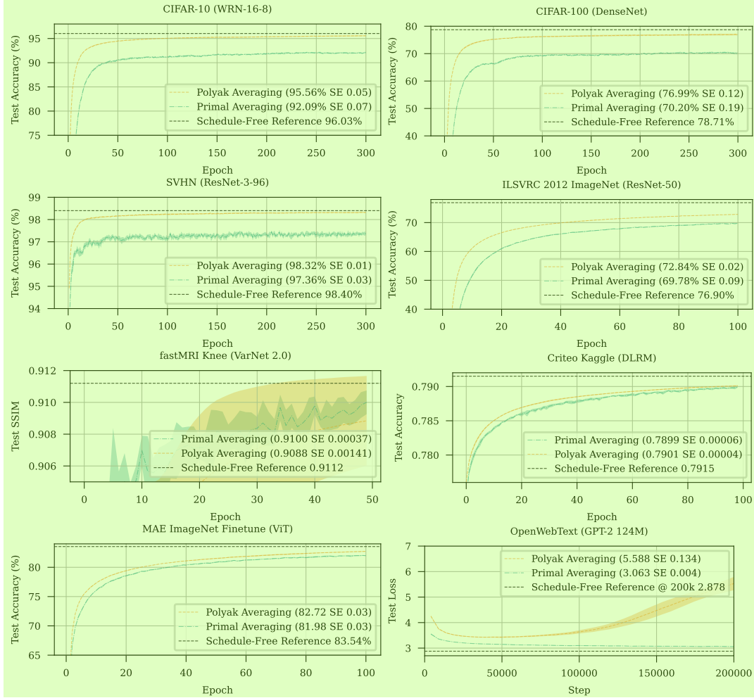
Figure 8: Polyak and Primal Averaging Experiments 4
