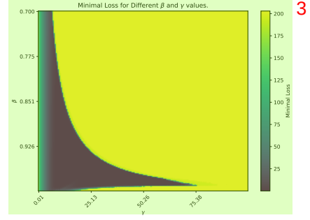
(b) Incorporating the momentum parameter \beta allows for convergence despite using larger learning rates \gamma on quadratic problems.
