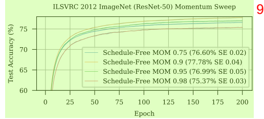
Figure 5: Sensitivity to momentum values
