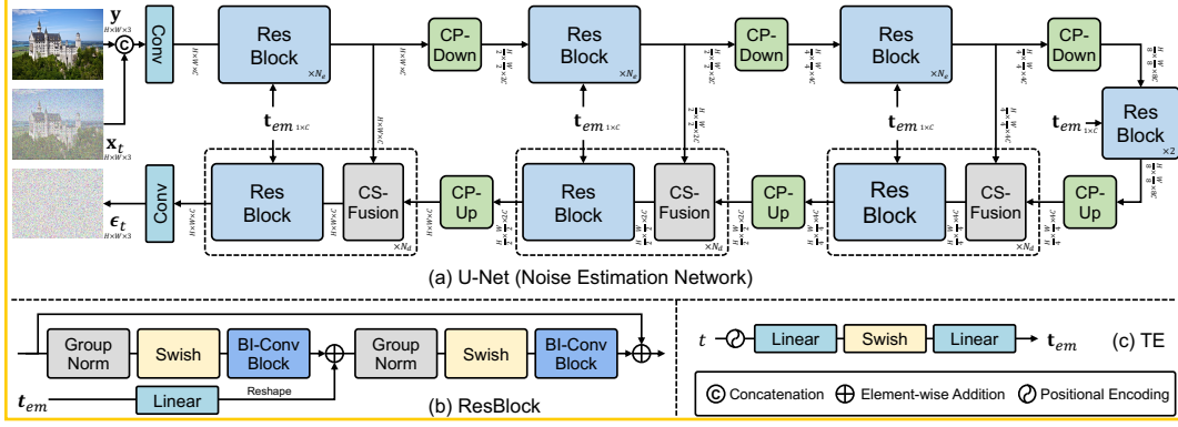
Figure 2: The overall structure of the noise estimation network. (a) UNet: The model consists of ResBlock, CP-Down, CP-Up, and CS-Fusion. It predicts noise \epsilon_t with the upsampled LR image y , noise image x_t , and timestep t . (b) ResBlock: Residual block, utilizes the binarized convolution (BI-Conv) block. The input and output dimensions of the block remain consistent, making it suitable for binarization. (c) TE: Time encoding, encodes timestep t to produce the timestep embedding t_{em} .
