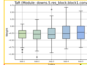
Figure 7: Weights of biases \mathbf{b}^j ( i \in \{1, \dots, 5\} ) in TaR.
