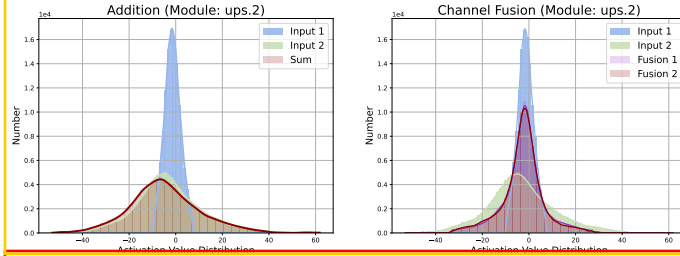
Figure 6: Activation distribution in the skip connection. Input 1(2): \mathbf{x}_1, \mathbf{x}_2 . Sum: \mathbf{x}_1 + \mathbf{x}_2 . Fusion 1(2): \mathbf{x}_1^{s/n}, \mathbf{x}_2^{s/n} .
