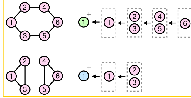
Figure 7. GRED provides distinct updates for the two graphs above. Such graphs, however, are indistinguishable by the 1-WL isomorphism test, assuming (worst-case) nodes have identical features.
