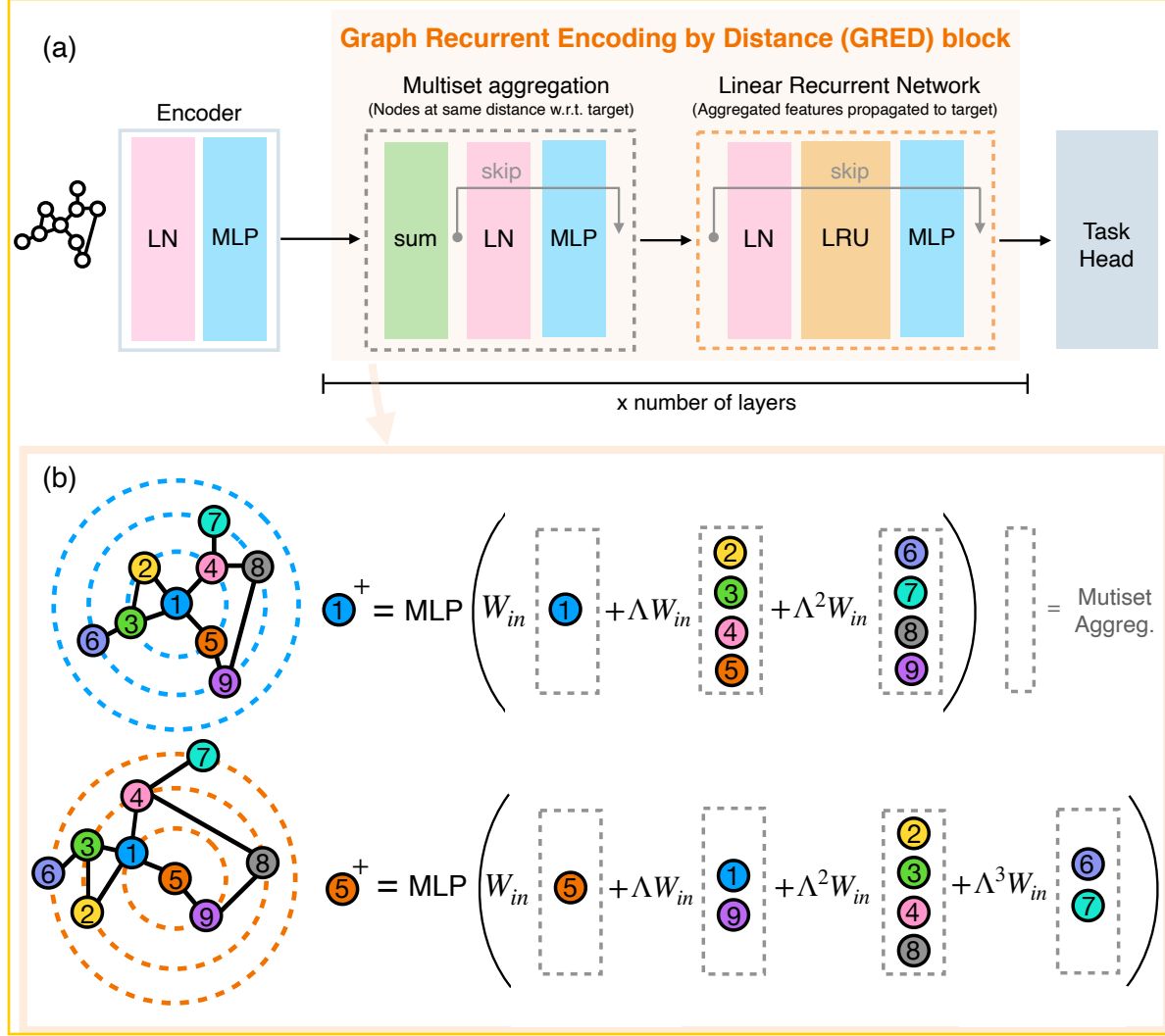
Figure 2. (a) Sketch of the architecture. MLPs and Layer Normalization operate independently at each node or aggregated multiset. Information of the distant nodes is propagated to the target node through a linear RNN – specifically an LRU (Orvieto et al., 2023b). (b) Depiction of the GRED layer operation for two different target nodes. The gray rectangular boxes indicate the application of multiset aggregation. Finally, the new representation for the target node is computed from the RNN output through an MLP.
