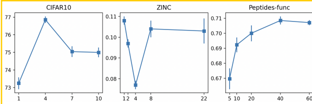
Figure 4. Effect of K on performance.
