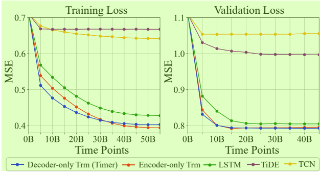
Figure 12. Training loss of candidate backbones. Model dimension and layer number are consistently chosen for a fair comparison.
