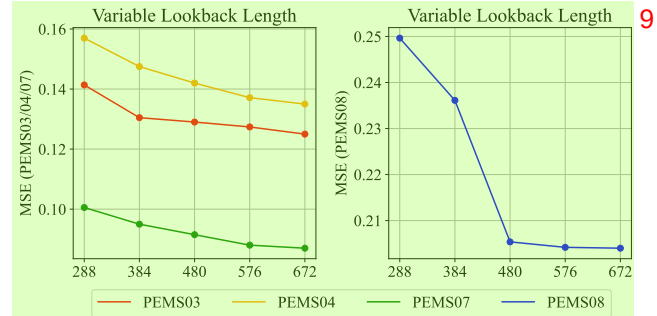
Figure 13. Performance of one Timer for all lookback lengths.
