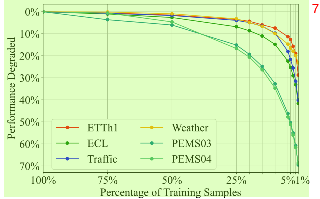
Figure 1. Performance of PatchTST (2022) on different data scarcities. The degradation is reported as the relative increase in MSE compared with training on full samples.
