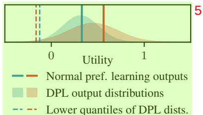
Figure 4: A comparison of how DPL and normal preference learning evaluate two responses to a jailbreak prompt. Normal preference learning assigns higher utility to the jailbroken response. While DPL also assigns a higher mean utility to the unsafe response, it also assigns it higher variance , indicating there is disagreement resulting from the helpfulness and harmlessness objectives diverging. Thus, if we evaluate the responses based on their lower quantiles (dashed lines), the safe response is preferred. 6
