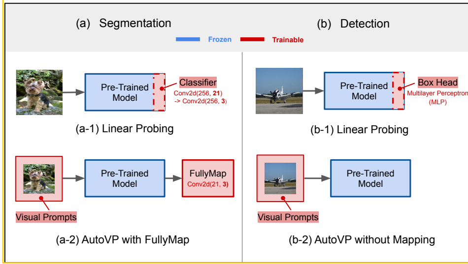
Figure E.2: LP and AutoVP in Segmentation and Detection Tasks.
