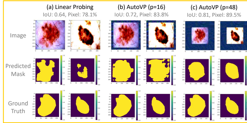
Figure E.3: ISIC Segmentation. Performance of LP and AutoVP with different prompt sizes (p). It's important to note that the performance calculation involves only the target image itself without the prompts, ensuring a fair comparison to LP. Specifically, the predicted mask is initially cropped to the region of the original target image and then resized to match the dimensions used in LP.
