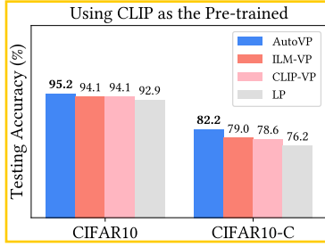
Figure 4: Models Robustness with CLIP. The comparison of accuracy drop on the CIFAR10-C dataset across AutoVP, ILM-VP, CLIP-VP and LP.
