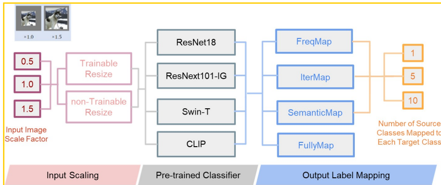
Figure A.2: Hyper-Parameter Tuning Selection. Illustration of the end-to-end hyper-parameter tuning process in AutoVP with a total of 222 possible configurations.
