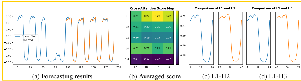
Figure 12: Illustration of (a) forecasting result, (b) averaged cross-attention score, and (c,d) patches with the highest score on Electricity. The score map is averaged from all the heads across layers.
