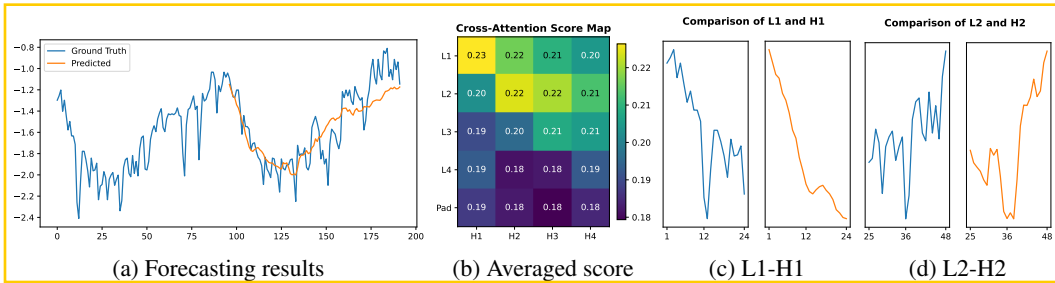
Figure 13: Illustration of (a) forecasting result, (b) averaged cross-attention score, and (c,d) patches with the highest score on ETTm2. The score map is averaged from all the heads across layers.
