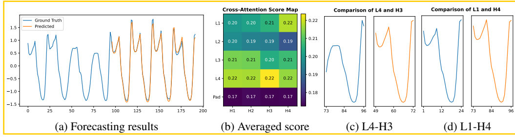
Figure 11: Illustration of (a) forecasting result, (b) averaged cross-attention score, and (c,d) patches with the highest score on Traffic. The score map is averaged from all the heads across layers.
