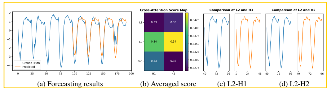
Figure 14: Illustration of (a) forecasting result, (b) averaged cross-attention score, and (c,d) patches with the highest score on ETTh1. The score map is averaged from all the heads across layers.
