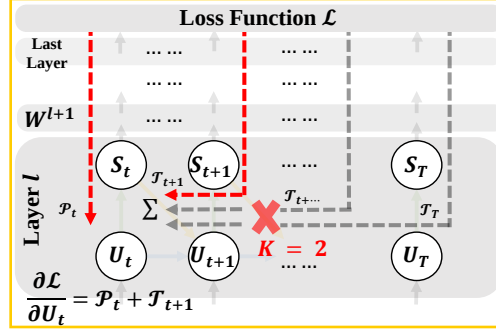
Figure 5. Illustration of the LIF neuron based SNN's gradient error flow during BPTT. In this example k=2 only the backpropagation from the first two timestep is considered (illustrated by the two red dashed arrows), and backpropagation along further timestep is discarded.
