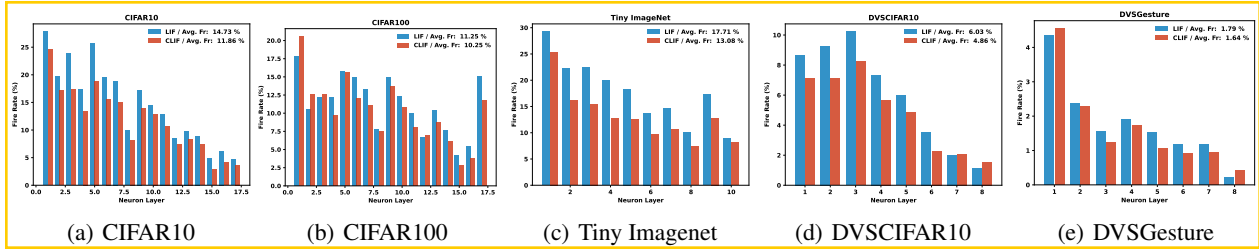
Figure 11. The fire rate statistics after training of LIF-based and CLIF-based for each tasks.
