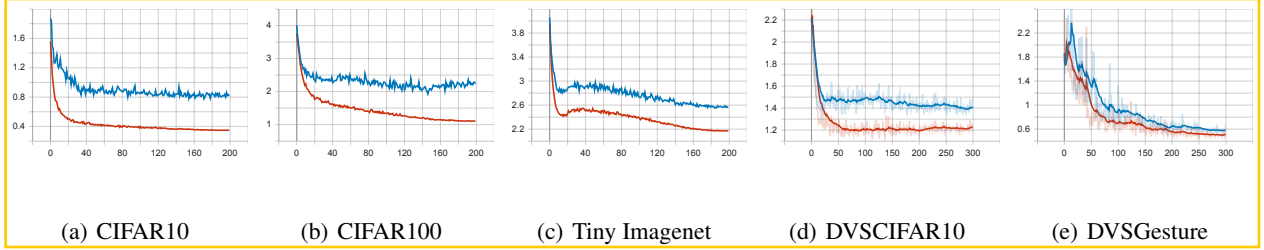
Figure 10. Testing loss curves of the training process of LIF-based and CLIF-based for each tasks.
