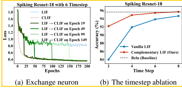
Figure 3. (a) Loss function vs epochs. Each color presents a case of either LIF, CLIF, or exchanging from LIF to CLIF at a given epoch during training. (b) Comparison of the accuracy of LIF and CLIF at various timestep. Both experiments are evaluated on the CIFAR10 task with Spiking ResNet-18.
