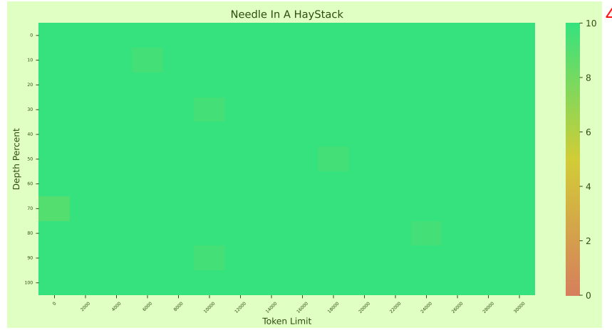
Figure 7: Performances of FILM-7B on Needle-in-the-Haystack. 5
