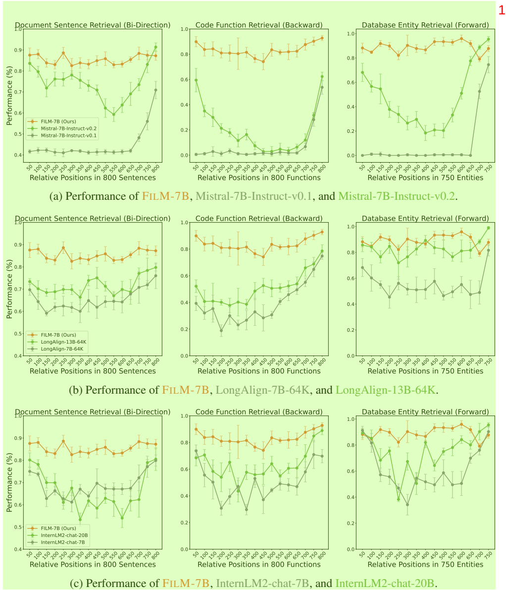
Figure 4: Performance of FILM-7B on VAL Probing and the comparisons with (a) Mistral, (b) LongAlign, and (c) InternLM2. The X-axis is the relative position in the context ( \sim 32K tokens).
