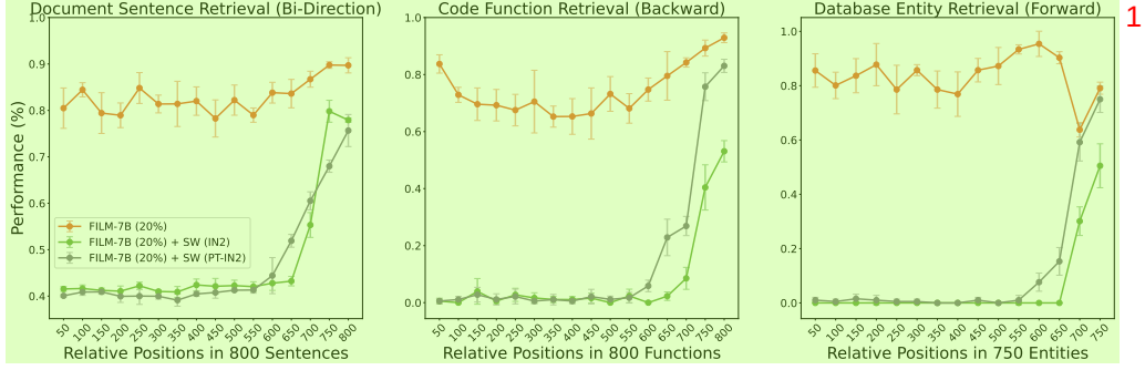
Figure 8: Performance of FILM-7B with a 4K sliding window (SW). PT-IN2: apply the sliding window in both pre-training and IN2 training. IN2: apply the sliding window only in IN2 training.
