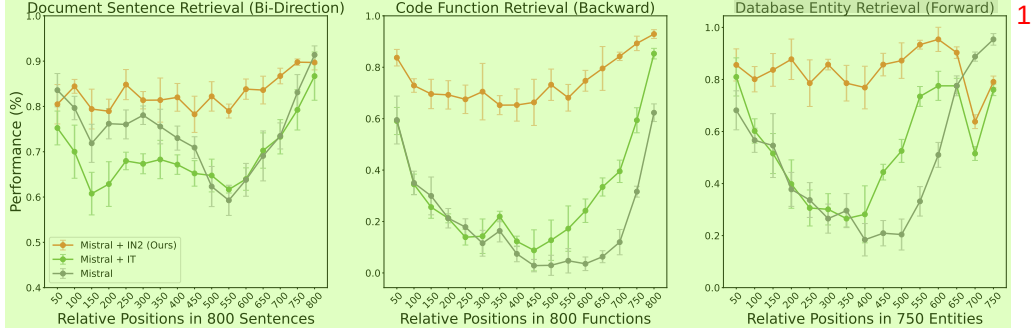
Figure 5: Compare the performance of IN2 training and general instruction tuning (IT). Both two training process takes the same number of training instances (20% of the full data size, 300K examples). Compare with Mistral + IN2 training, the gains from normal instruction tuning are marginal and unstable.
