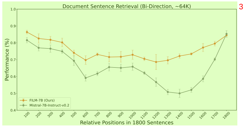
Figure 9: Performance of FILM-7B on 64K context length. The position embeddings are extended 4 through YaRN.
