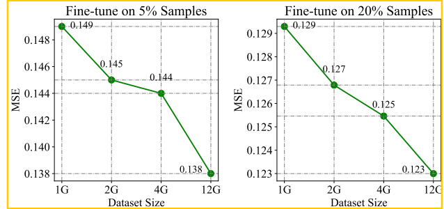
Figure 11. Timer trained on larger dataset demonstrates better performance on downstream forecasting. Models are configured with L = 8 and D = 1024 . Detailed results are provided in Table 16.
