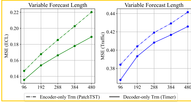
Figure 15. Performance of Timer/PatchTST for all forecast lengths. We conduct rolling forecasting on a single 672-pred-96 model.
