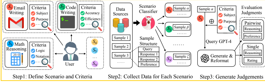
Figure 1: An overview for our data construction pipeline in three steps.
