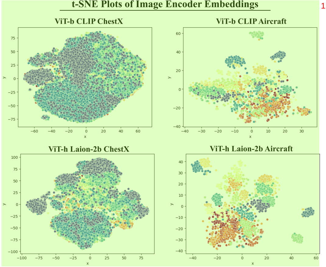
Figure 4: t-SNE projections of different image embeddings of various benchmark datasets with embeddings colored class identity. We see ViT-huge trained with Laion-2b better separates the Aircraft dataset than does ViT-base trained with CLIP. However, both image encoders are unable to separate ChestX.
