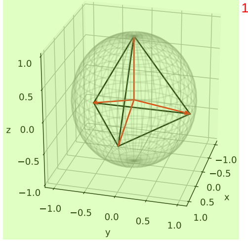
Figure 3: A visualization of a d = 4 ELMES in \mathbb{R}^3 . Observe the endpoints of the vectors of an ELMES lie on the vertices of a centered regular tetrahedron.
