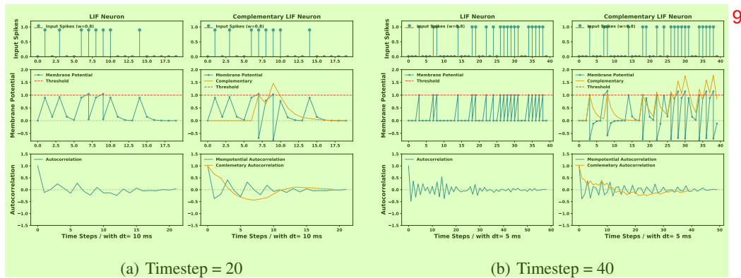
Figure 8. The autocorrelation of a single LIF and CLIF neuron at different timestep.
