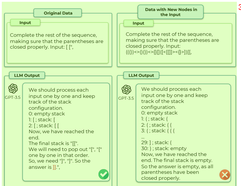
Figure 17: A case study on the BBH Dyck Language dataset wherein GPT-3.5 Turbo accurately generates the correct answer but errs on the modified data with increased complexity using DARG. 4
