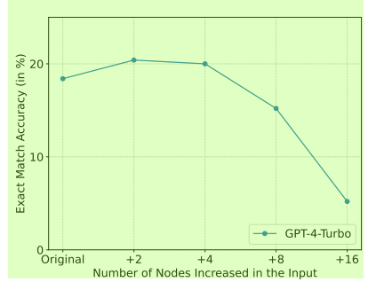
Figure 8: Performance of GPT-4 Turbo on the BBH Dyck language using least-to-most prompting as the number of nodes in the input increases. 5
