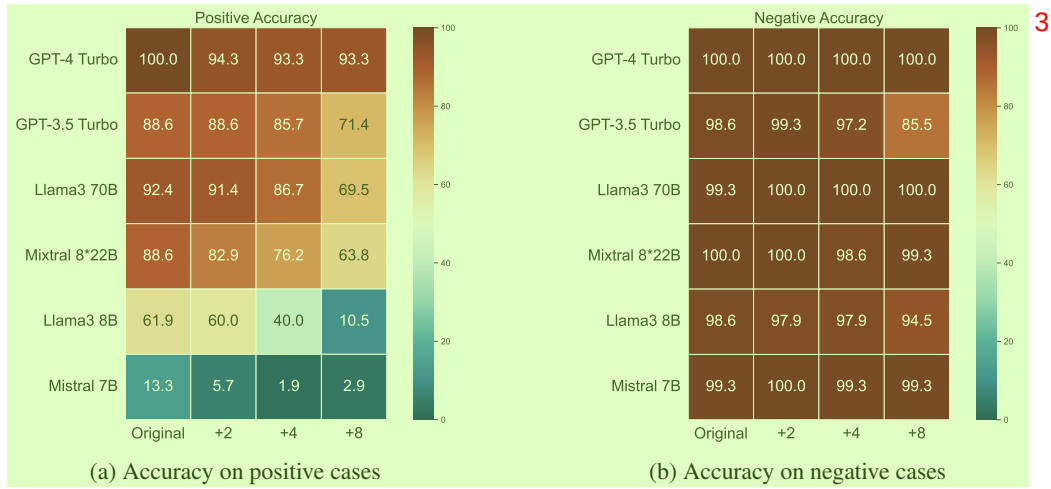
Figure 12: Performance of different LLMs as complexity increases through DARG in positive and negative cases on BBH Navigate using CoT. 4
