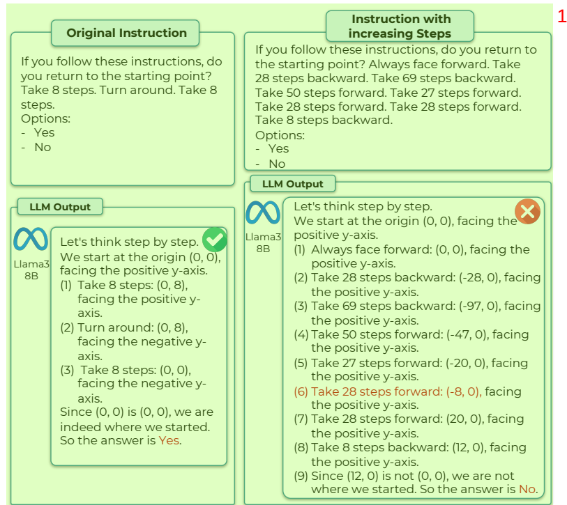
Figure 16: A case study on the BBH Navigate dataset wherein Llama-3-8B accurately generates the correct answer but errs on the modified data with increased complexity using DARG. 2
