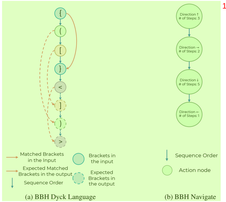
Figure 11: Examples of reasoning graphs for the two tasks we evaluate in BBH. 2
