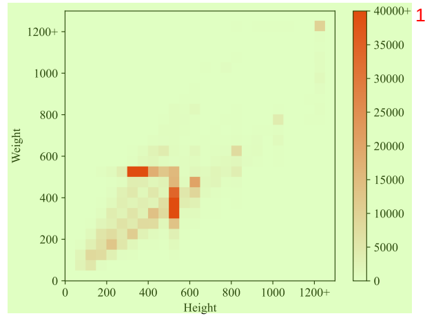
Figure 4: Height/Width distribution of the original ImageNet (Deng et al., 2009) dataset. 2
