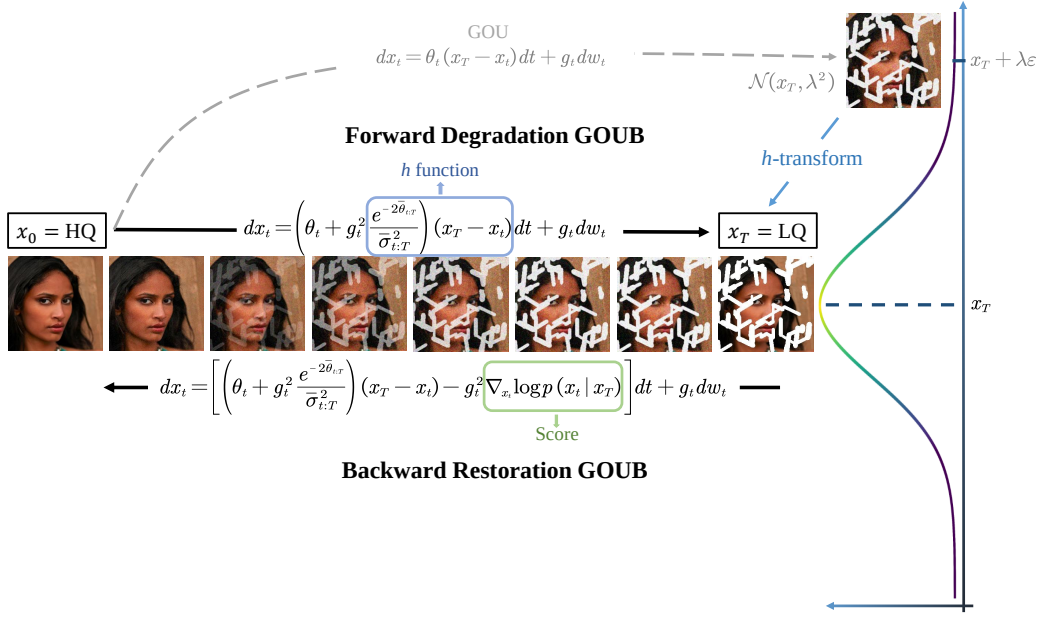
Figure 1. Overview of the proposed GOUB for image restoration. The GOU process is capable of transferring an HQ image into a noisy LQ image. Additionally, through the application of h -transform, we can eliminate the noise on LQ, enabling the GOUB model to precisely bridge the gap between HQ and LQ.
