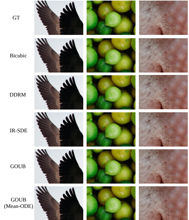
Figure 4. Qualitative comparison of the visual results of different 4x super-resolution methods on the DIV2K dataset.
