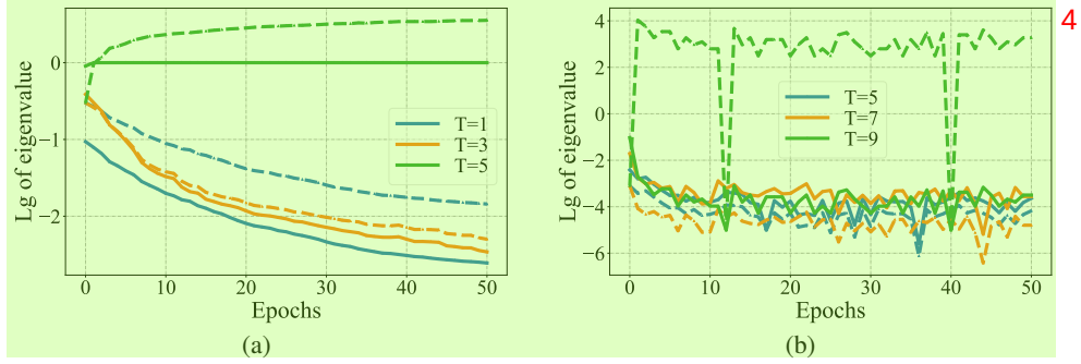
Figure 6: Investigate the spectrum of transformed output \hat{\mathbf{Z}} (solid lines) and the corresponding embedding \mathbf{Z} (dashed lines) using IterNorm for SSL with different iteration numbers T . We show the evolution of eigenvalues during training on the toy 2D dataset (Note that there are only two eigenvalues and we ignore the larger one because it always remains a high value during training). In particular, (a) shows the results with a well-conditioned initial spectrum while (b) with a ill-conditioned one.
