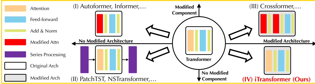
Figure 3: Transformer-based forecasters categorized by component and architecture modifications.
