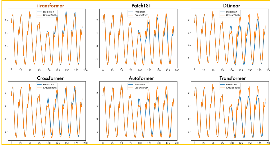
Figure 13: Visualization of input-96-predict-96 results on the Traffic dataset.
