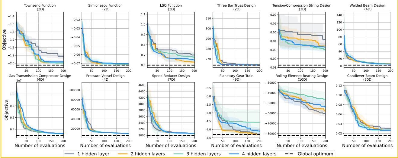
Figure 15: Comparison of BE-CBO with different number of hidden layers for the Deep Ensemble classifier. The current best value is shown w.r.t. the number of function evaluations. The curve is averaged over 10 different initial random seeds. The performance of BE-CBO is not particularly sensitive to the number of layers as long as it has more than one hidden layer.
