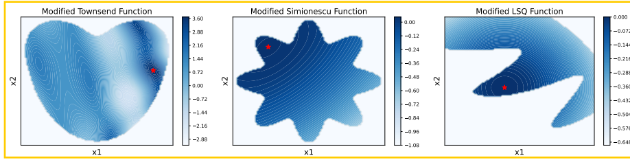
Figure 10: Landscape of the modified Townsend, Simionescu and LSQ functions. The red star indicates the global optimum location, which is inside the feasible region instead of on the constraint boundary in their original forms.
