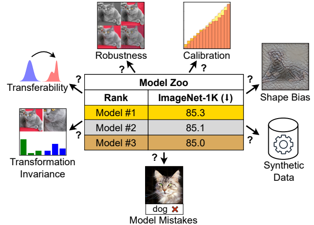
Figure 1. Models are often compared only by their ImageNet accuracy, without looking at many other important behaviors. In our work, we analyze models with similar ImageNet accuracies and find that they have vastly different properties.
