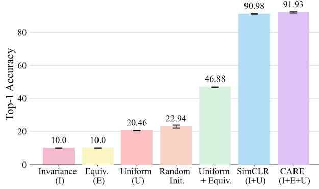
Figure 10: Ablating different loss terms. Combining \mathcal{L}_{\text{equi}} with a uniformity promoting non-collapse term suffices to learn non-trivial features. However, optimal performance is achieved when encouraging smaller rotations, as in CARE. ResNet-50 models pretrained on CIFAR10 and evaluated with linear probes.
