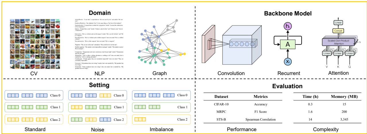
Figure 1. CurBench includes 15 datasets spanning 3 research domains, 9 backbone models, 3 training settings, and 2 evaluation dimensions, providing a comprehensive benchmark for existing curriculum learning methods.
