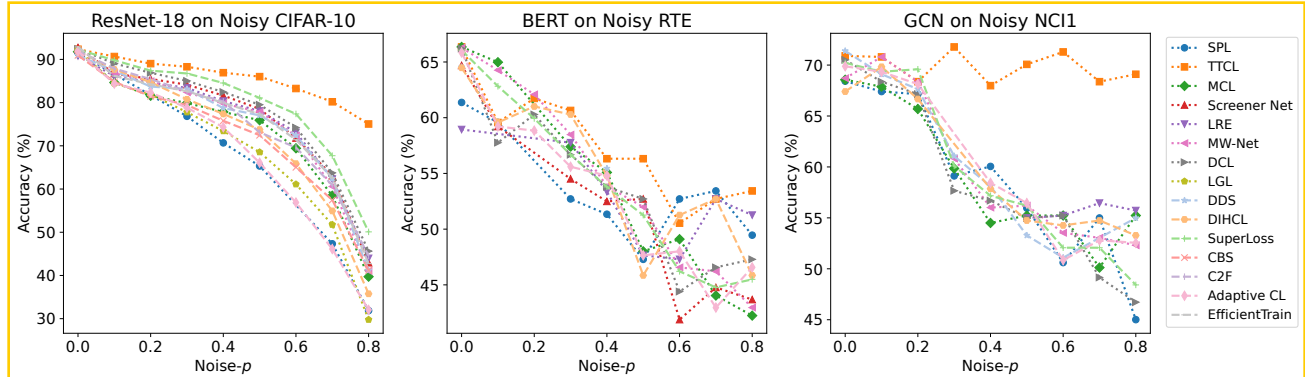
Figure 4. The performances as a function of noise ratio for different curriculum learning methods on datasets from 3 research domains.
