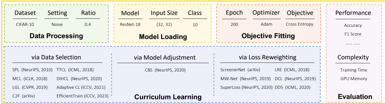
Figure 2. Our CurBench toolkit, which is composed of 5 modules, offers a unified and complete pipeline from initiation to evaluation, aiming for easy implementation and reproduction of curriculum learning methods. This figure showcases an example of noisy CIFAR-10.
